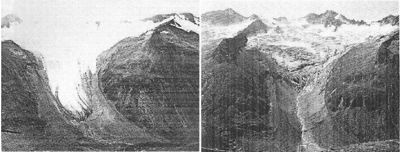
The glacier Waxeckkees in Zemmgrund, Zillertaler Alpen, Austria, in August 1921 (left; photo by S. Ulrich or R. Finsterwalder) and in 8 September 1973 (right; photo by H. Rentsch). The large 1850 moraines are clearly seen on either side of the glacier. Reproduced from Heuberger 1977.
