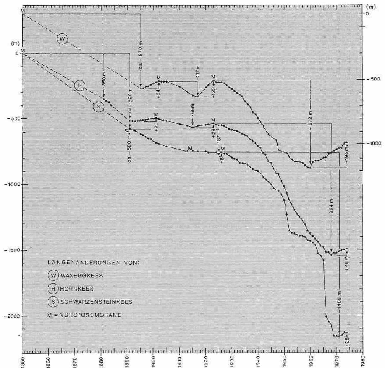
Diagram showing frontal retreat (in meters) of the three glaciers Waxeggkees, Hornkees and Schwarzensteinkees in the valley Zemmgrund, Zillertaler Alpen, Austria, from the maximum Little Ice Age position reached around 1850. A period of rapid frontal retreat began around 1920, followed by a period of beginning advance from 1960-1970. Diagram reproduced from Heuberger 1977, originally published by Hoinkes et al. 1975.
