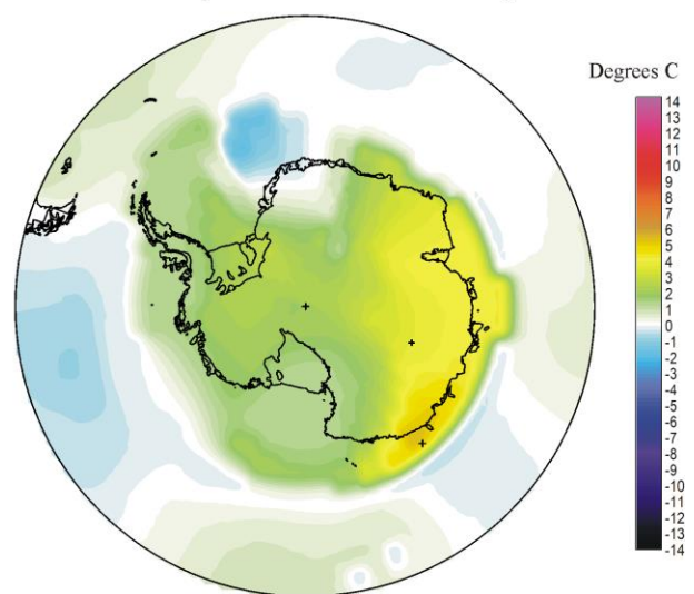
Air temperature 2018 04 versus last 10 yr
