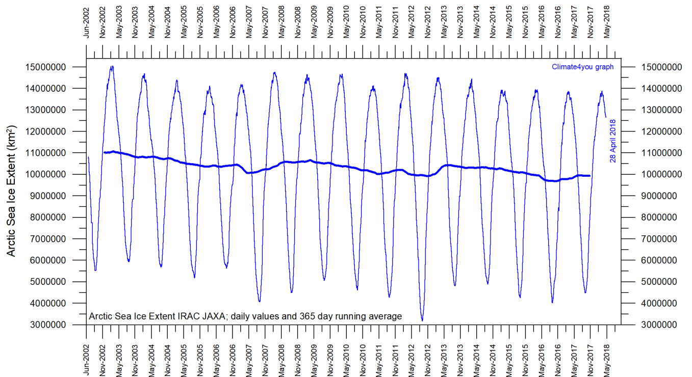
Diagram showing daily Arctic sea ice extent since June 2002, to 28 April 2018, by courtesy of Japan Aerospace Exploration Agency (JAXA).
