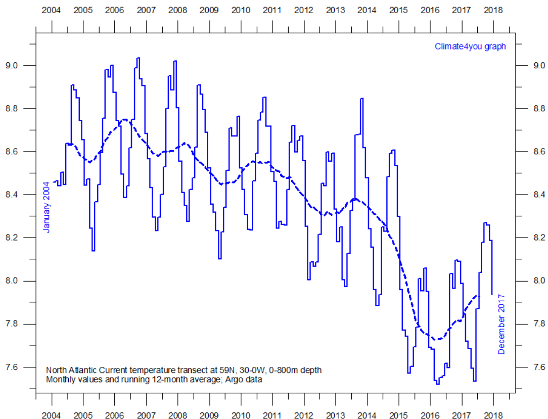
Average temperature along 59°N, 30-0°W, 0-800m depth, corresponding to the main part of the North Atlantic Current, using Argo -data. Source: Global Marine Argo Atlas . Additional information can be found in: Roemmich, D. and J. Gilson, 2009. The 2004-2008 mean and annual cycle of temperature, salinity, and steric height in the global ocean from the Argo Program. Progress in Oceanography , 82, 81-100.
