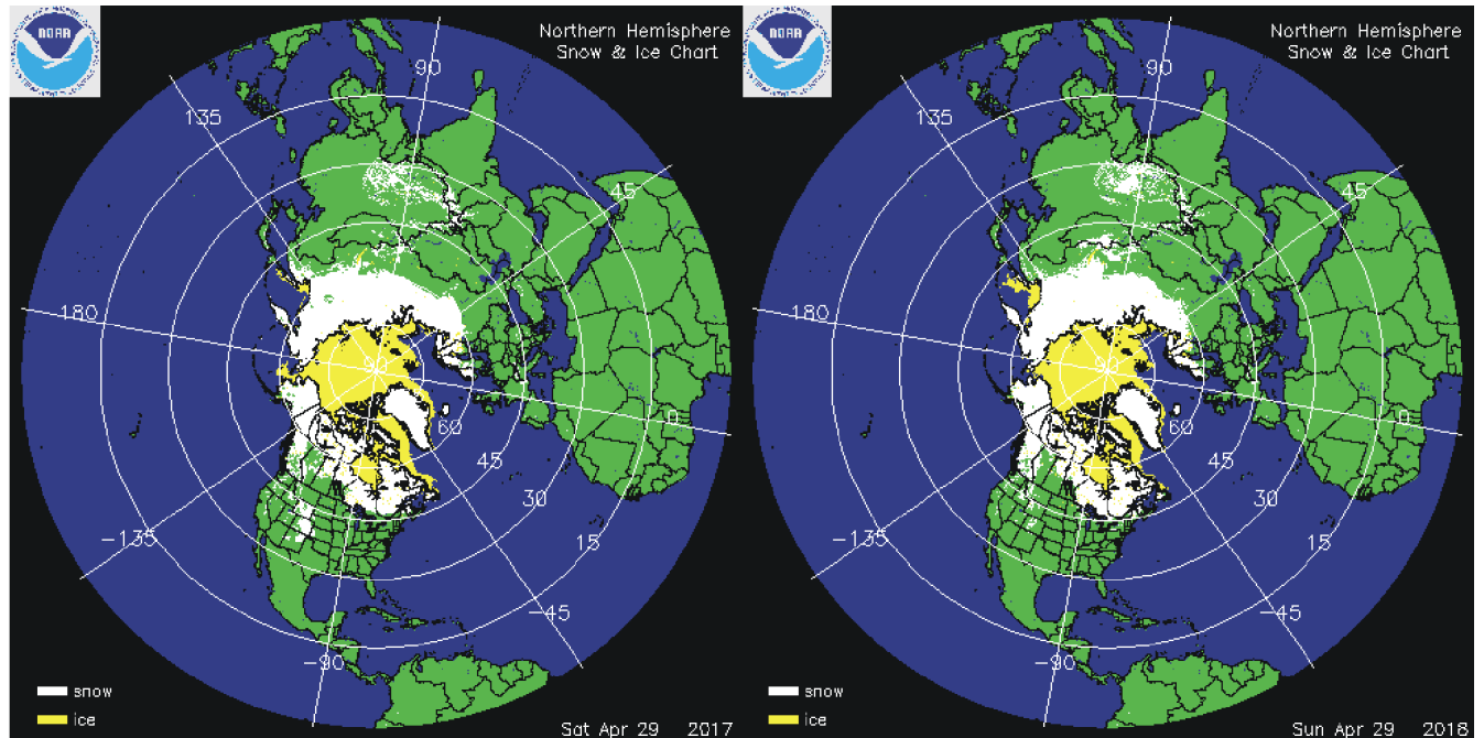
Northern hemisphere snow cover (white) and sea ice (yellow) 29 April 2017 (left) and 2018 (right). Map source: National Ice Center (NIC) .
