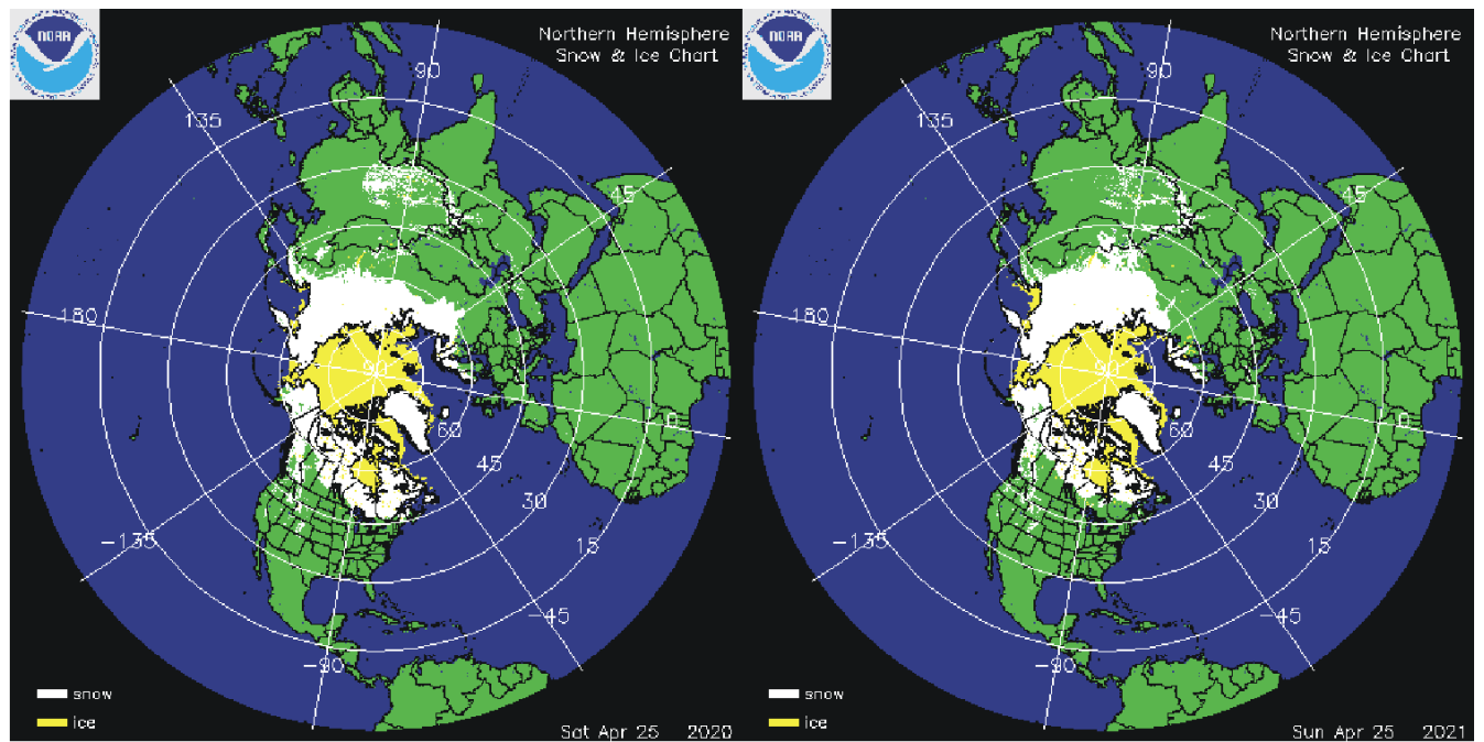
Northern hemisphere snow cover (white) and sea ice (yellow) 25 April 2020 (left) and 2021 (right). Map source: National Ice Center (NIC) .
