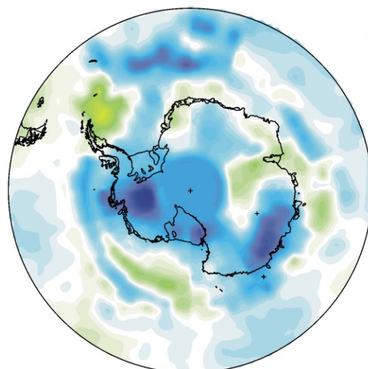
Surface air temperature April 2021 versus April last 10 yr
