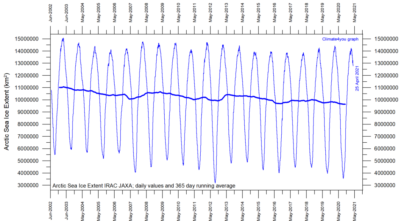
Diagram showing daily Arctic sea ice extent since June 2002, to 25 April 2021, by courtesy of Japan Aerospace Exploration Agency (JAXA).
