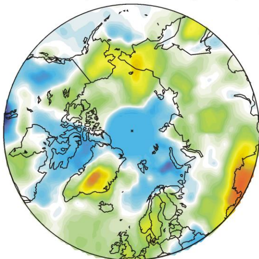
Surface air temperature April 2022 versus April last 10 yr
