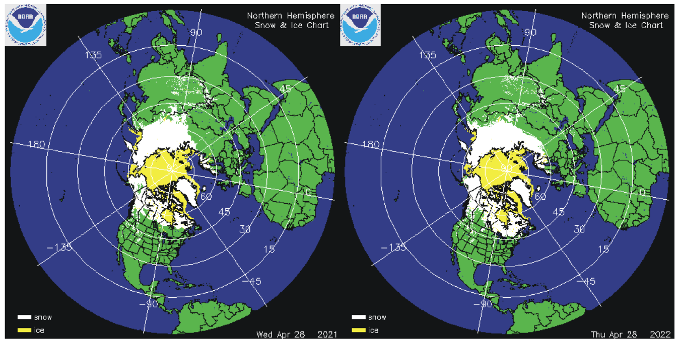
Northern hemisphere snow cover (white) and sea ice (yellow) 28 April 2021 (left) and 2022 (right). Map source: National Ice Center (NIC) .
