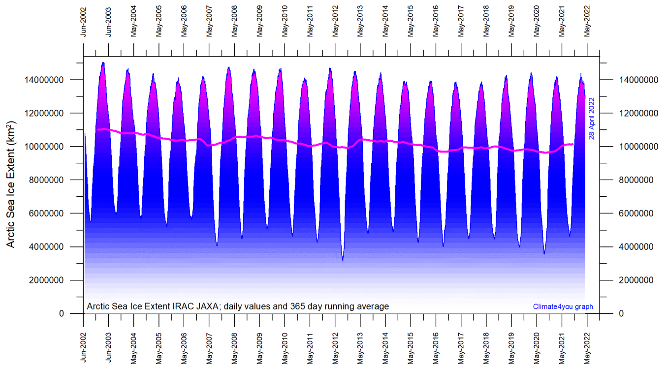
Diagram showing daily Arctic sea ice extent since June 2002, to 28 April 2022, by courtesy of Japan Aerospace Exploration Agency (JAXA).
