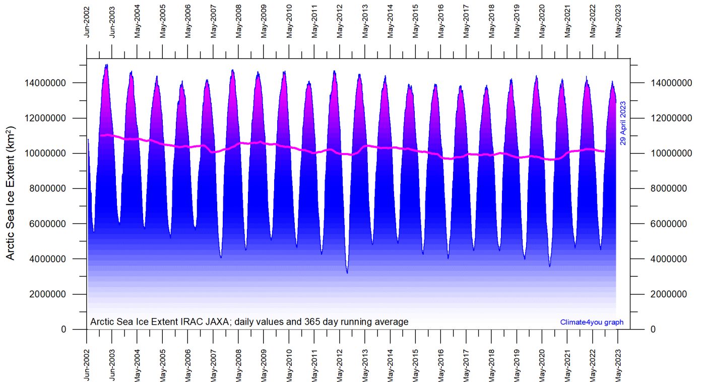
Diagram showing daily Arctic sea ice extent since June 2002, to 29 April 2023, by courtesy of Japan Aerospace Exploration Agency (JAXA) .
