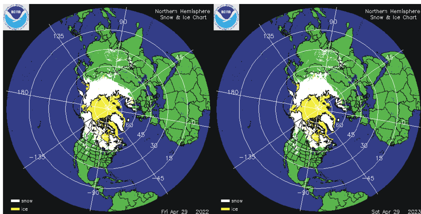
Northern hemisphere snow cover (white) and sea ice (yellow) 29 April 2022 (left) and 2023 (right). Map source: National Ice Center (NIC) .
