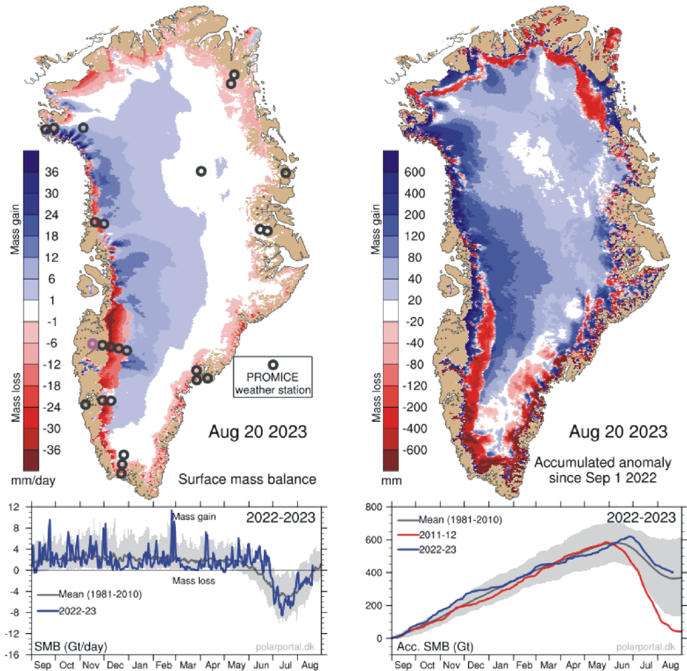
Left: Surface mass balance 20 August 2023. Right: Net surface mass balance anomaly since September 1, 2022. Courtesy of Danish Meteorological Institute (DMI).
