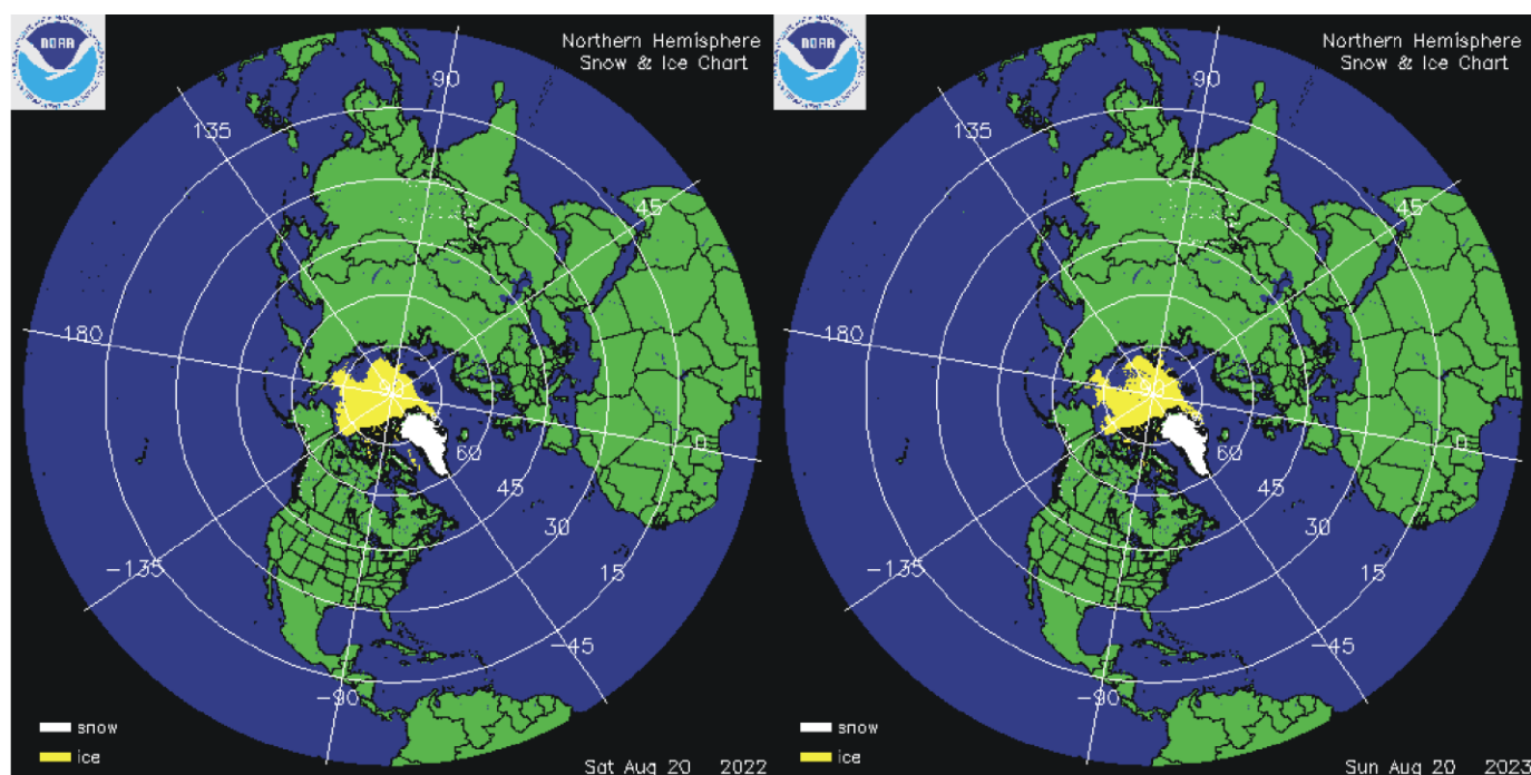
Northern hemisphere snow cover (white) and sea ice (yellow) 20 August 2022 (left) and 2023 (right). Map source: National Ice Center (NIC) .
