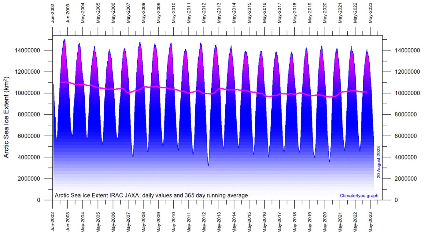
Diagram showing daily Arctic sea ice extent since June 2002, to 20 August 2023, data courtesy of Japan Aerospace Exploration Agency (JAXA) .
