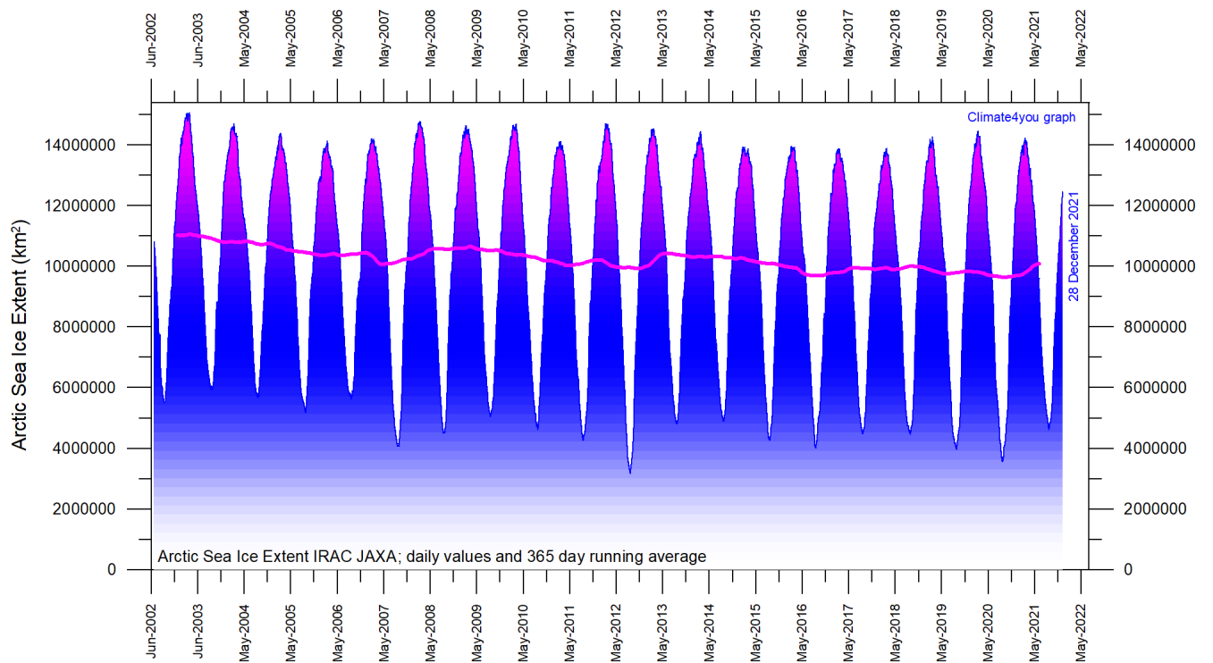
Diagram showing daily Arctic sea ice extent since June 2002, to 28 December 2021, by courtesy of Japan Aerospace Exploration Agency (JAXA).
