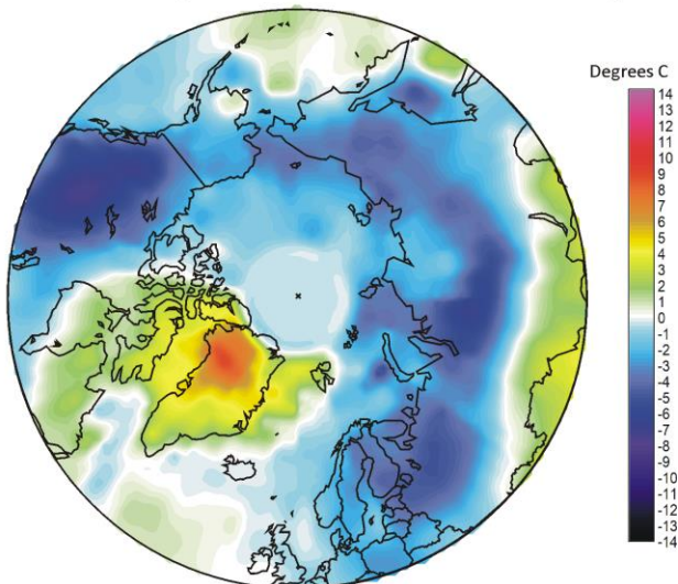
Surface air temperature December 2021 versus December last 10 yr
