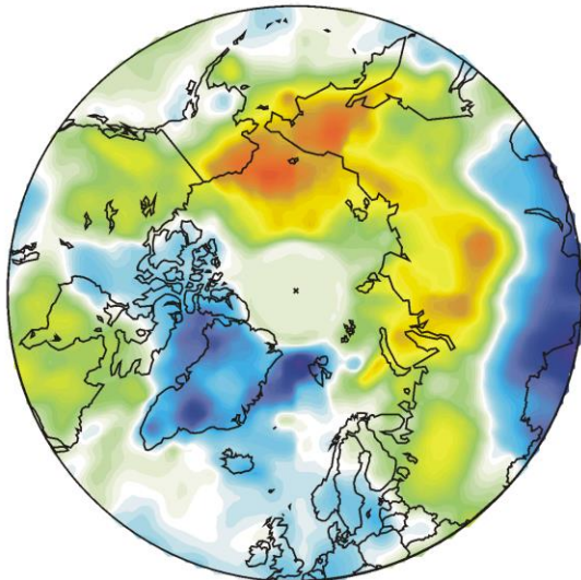
Surface air temperature December 2022 versus December 2021
