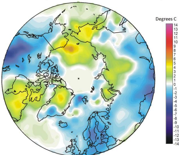
Surface air temperature December 2022 versus December last 10 yr
