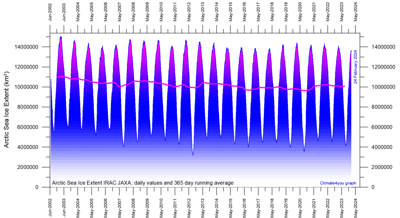
Diagram showing daily Arctic sea ice extent since June 2002, to 24 February 2024, data courtesy of Japan Aerospace Exploration Agency (JAXA) .
