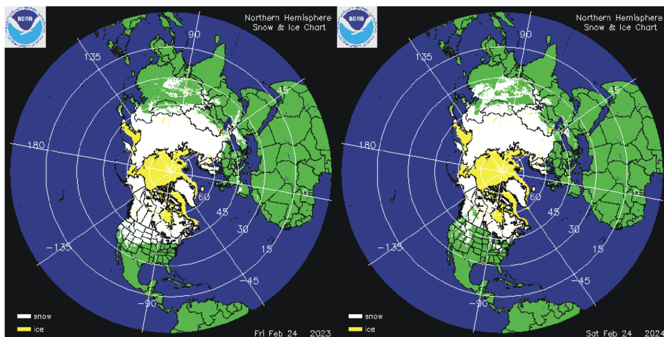
Northern hemisphere snow cover (white) and sea ice (yellow) 24 February 2023 (left) and 2024 (right). Map source: National Ice Center (NIC) .
