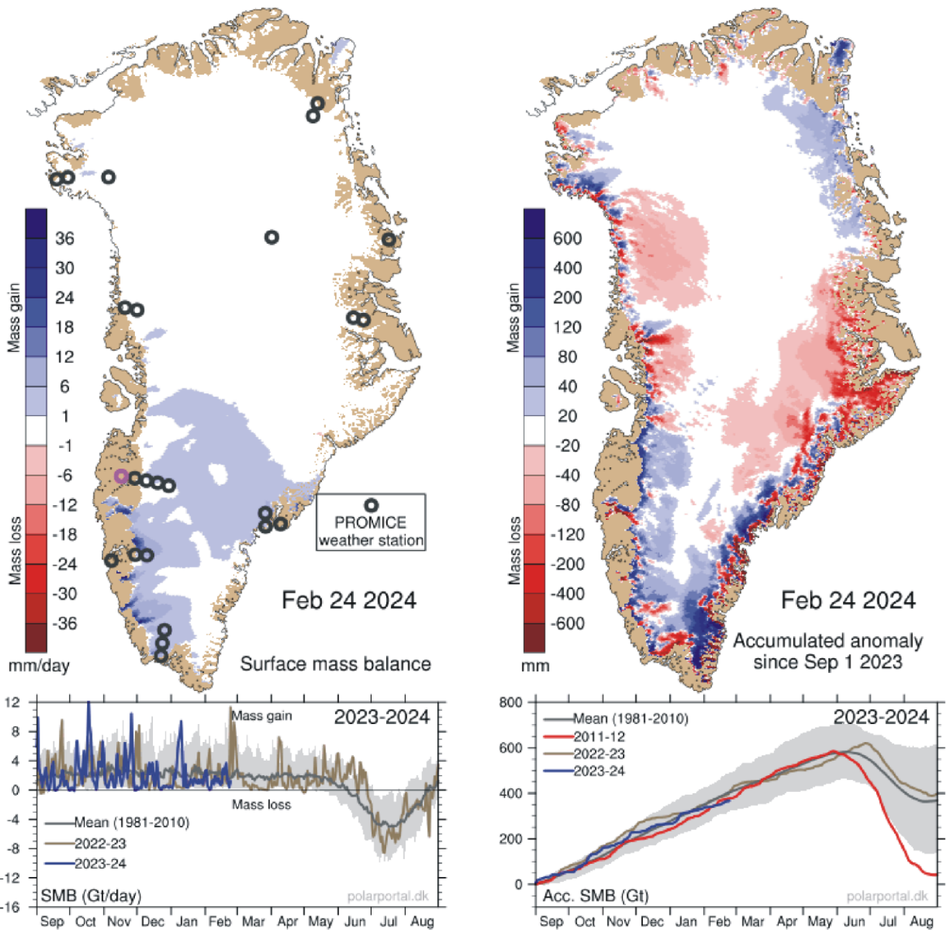
Left: Surface mass balance 24 February 2024. Right: Net surface mass balance anomaly since September 1, 2023. Courtesy of Danish Meteorological Institute (DMI).
