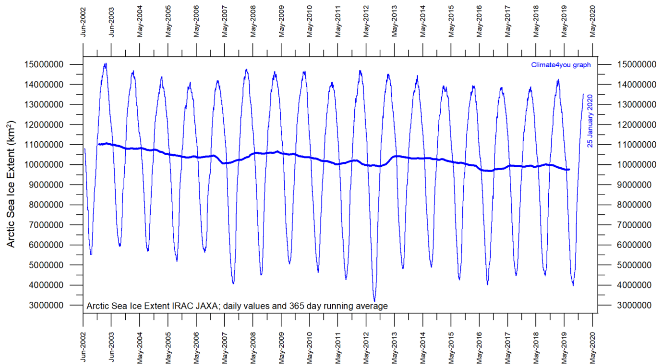
Diagram showing daily Arctic sea ice extent since June 2002, to 25 January 2020, by courtesy of Japan Aerospace Exploration Agency (JAXA).
