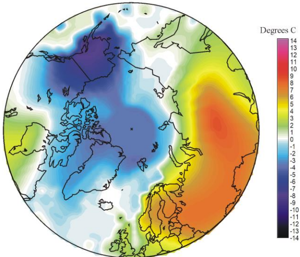
Surface air temperature January 2020 versus last 10 yr
