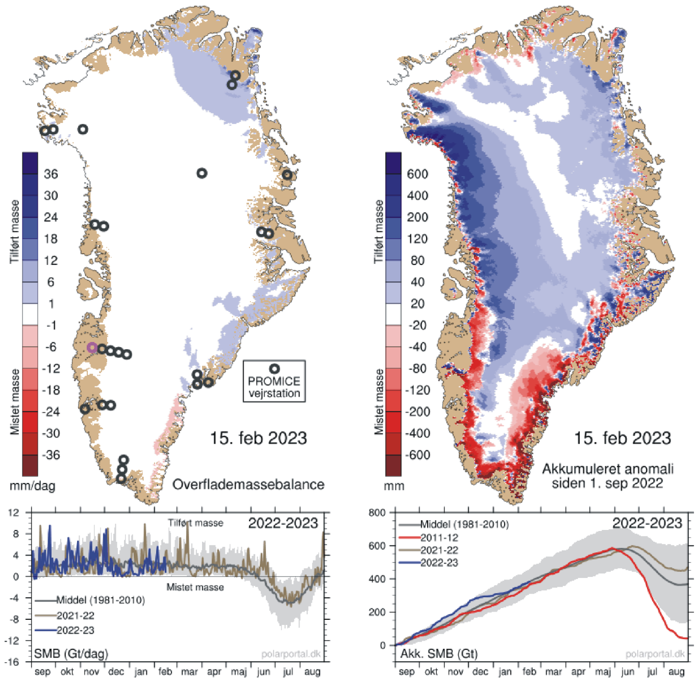
Left: Surface mass balance 15 February 2023. Right: Net surface mass balance anomaly since September 1, 2022. Courtesy of Danish Meteorological Institute (DMI).
