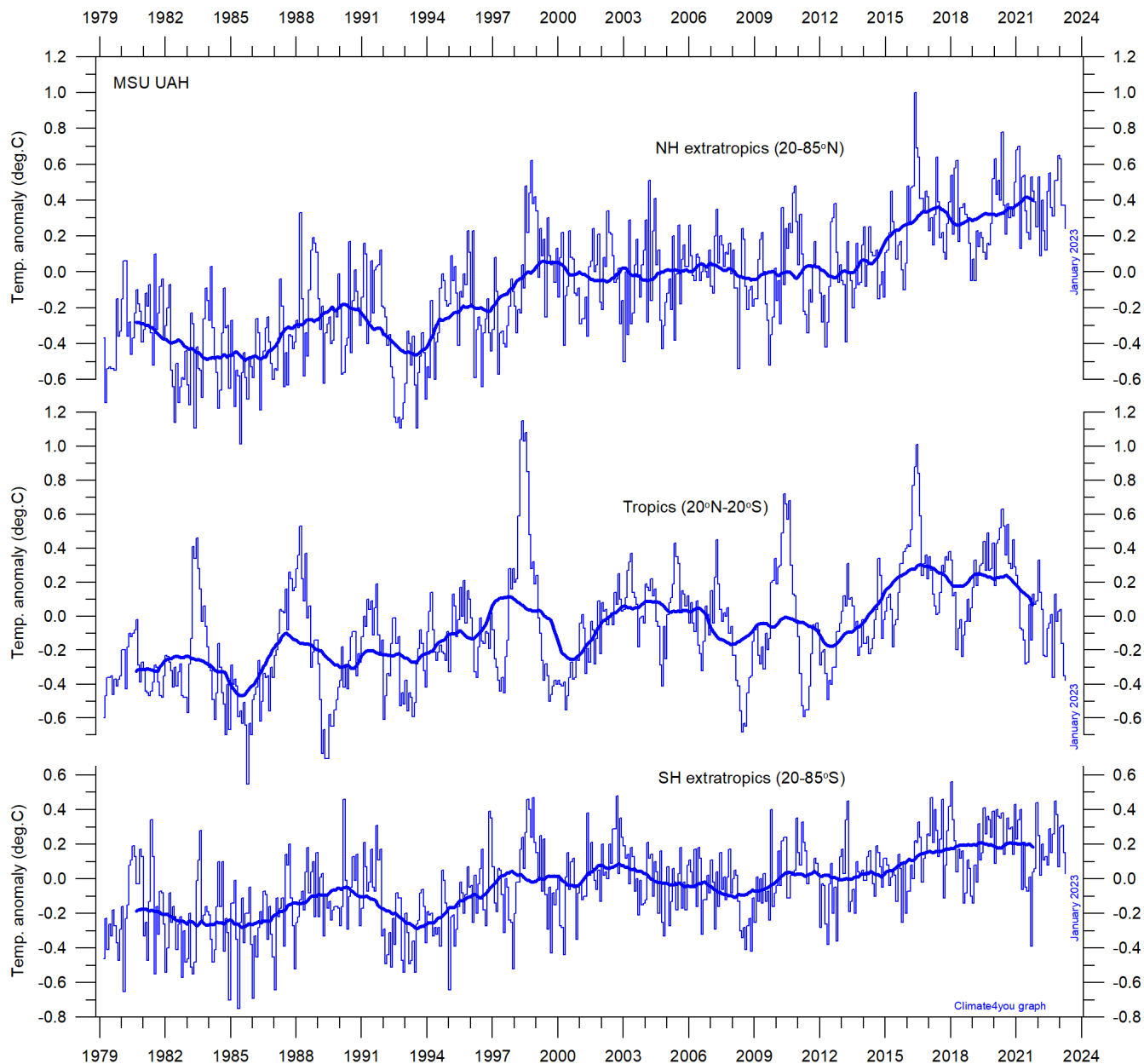
Global monthly average lower troposphere temperature since 1979 for the tropics and the northern and southern extratropics, according to University of Alabama at Huntsville, USA. Thin lines show the monthly temperature. Thick lines represent the simple running 37-month average, nearly corresponding to a running 3-year average. Reference period 1981-2010.
