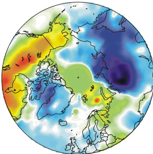
Surface air temperature January 2023 versus January 2022
