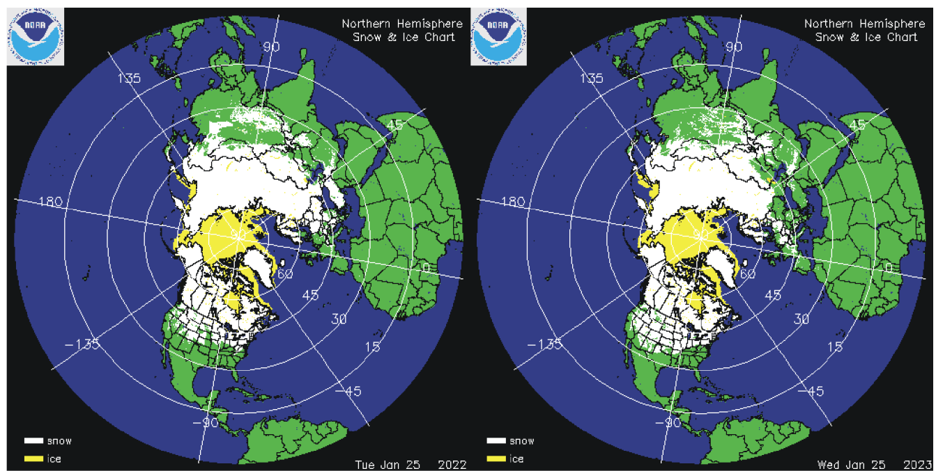
Northern hemisphere snow cover (white) and sea ice (yellow) 25 January 2022 (left) and 2023 (right). Map source: National Ice Center (NIC).
