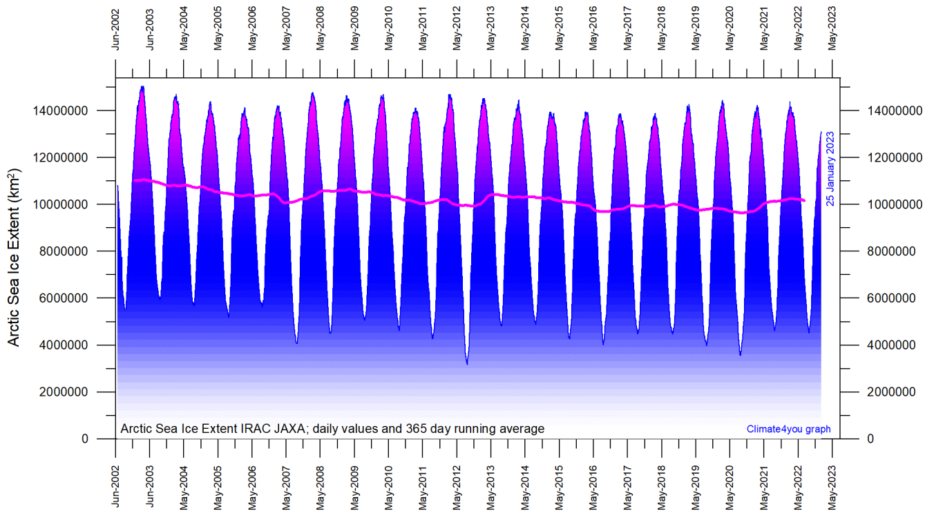
Diagram showing daily Arctic sea ice extent since June 2002, to 25 January 2023, by courtesy of Japan Aerospace Exploration Agency (JAXA).
