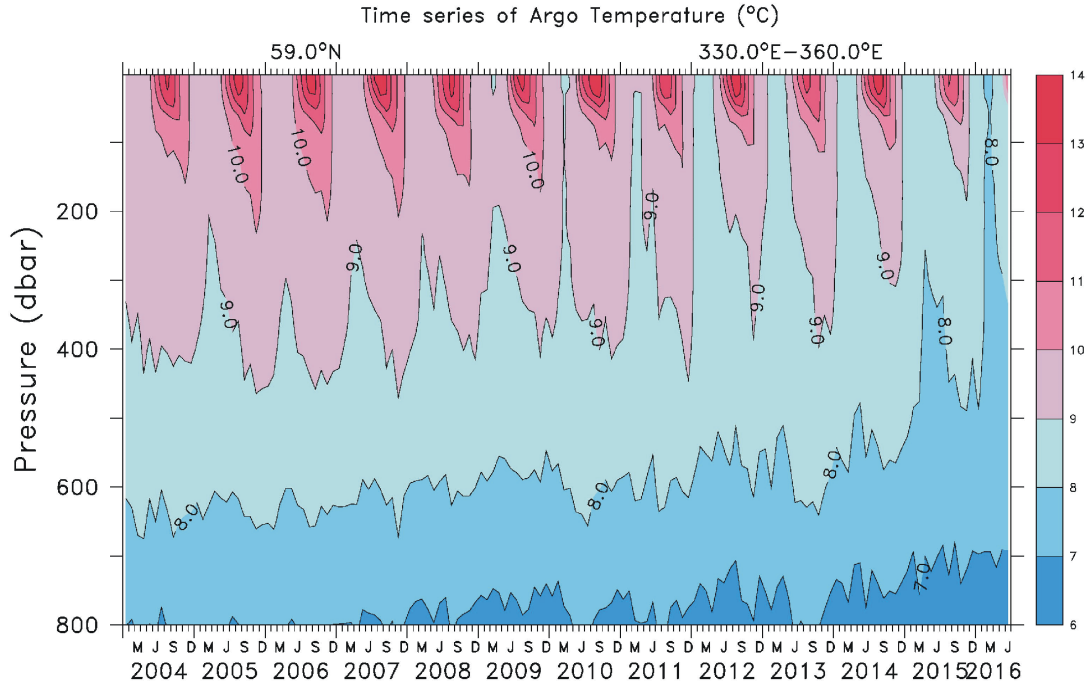
Time series depth-temperature diagram along 59 N across the North Atlantic Current from 30°W to 0°W, from surface to 800 m depth. Source: Global Marine Argo Atlas . See also the diagram below.
