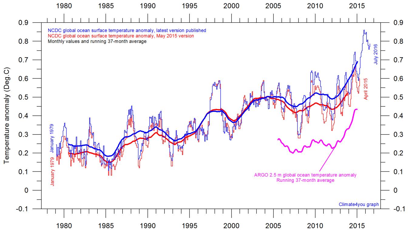
Global monthly average sea surface temperature since 1979 according to the National Climatic Data Center (NCDC), USA. Base period: 1901-2000. The thick line is the simple running 37-month average. Insert: Argo global ocean temperature anomaly from floats.
