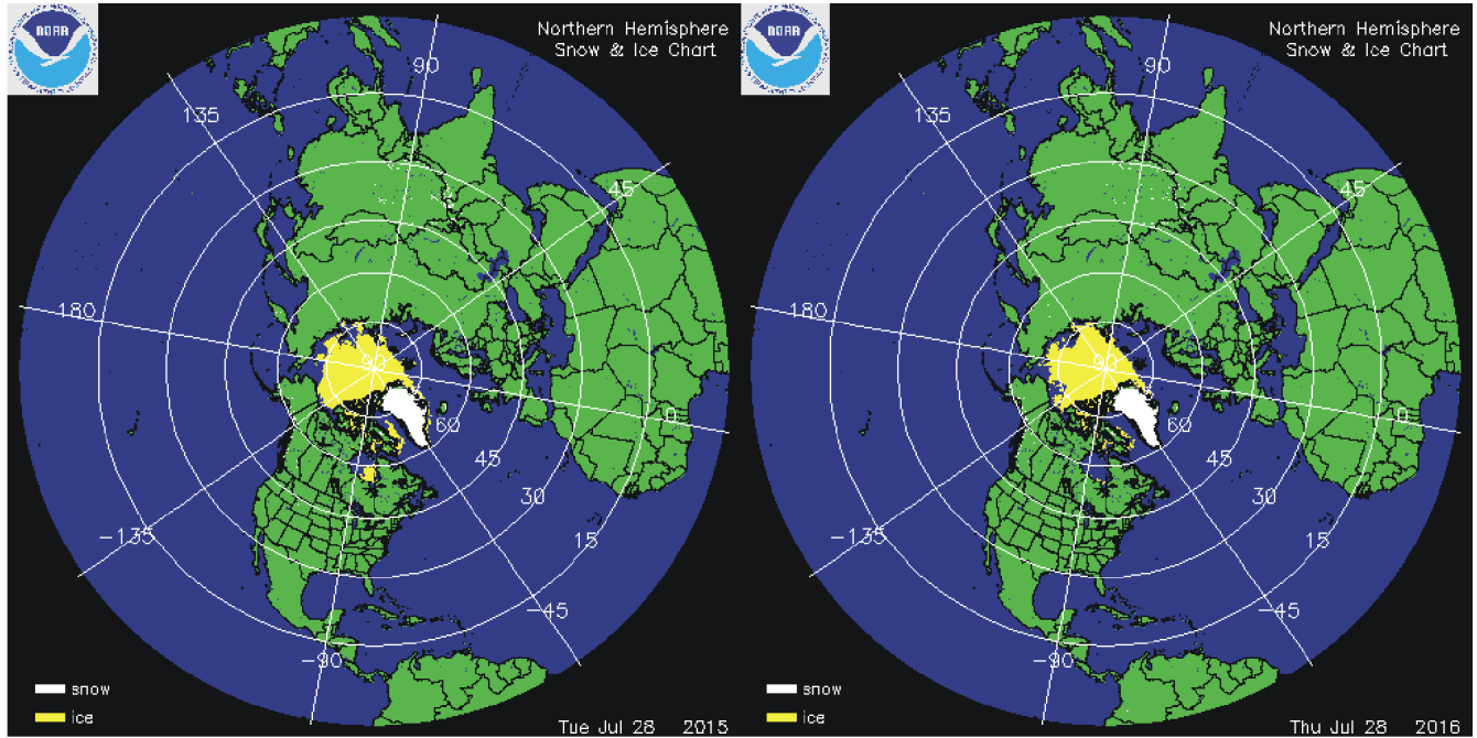
Northern hemisphere snow cover (white) and sea ice (yellow) 28 July 2015 (left) and 2016 (right). Map source: National Ice Center (NIC) .
