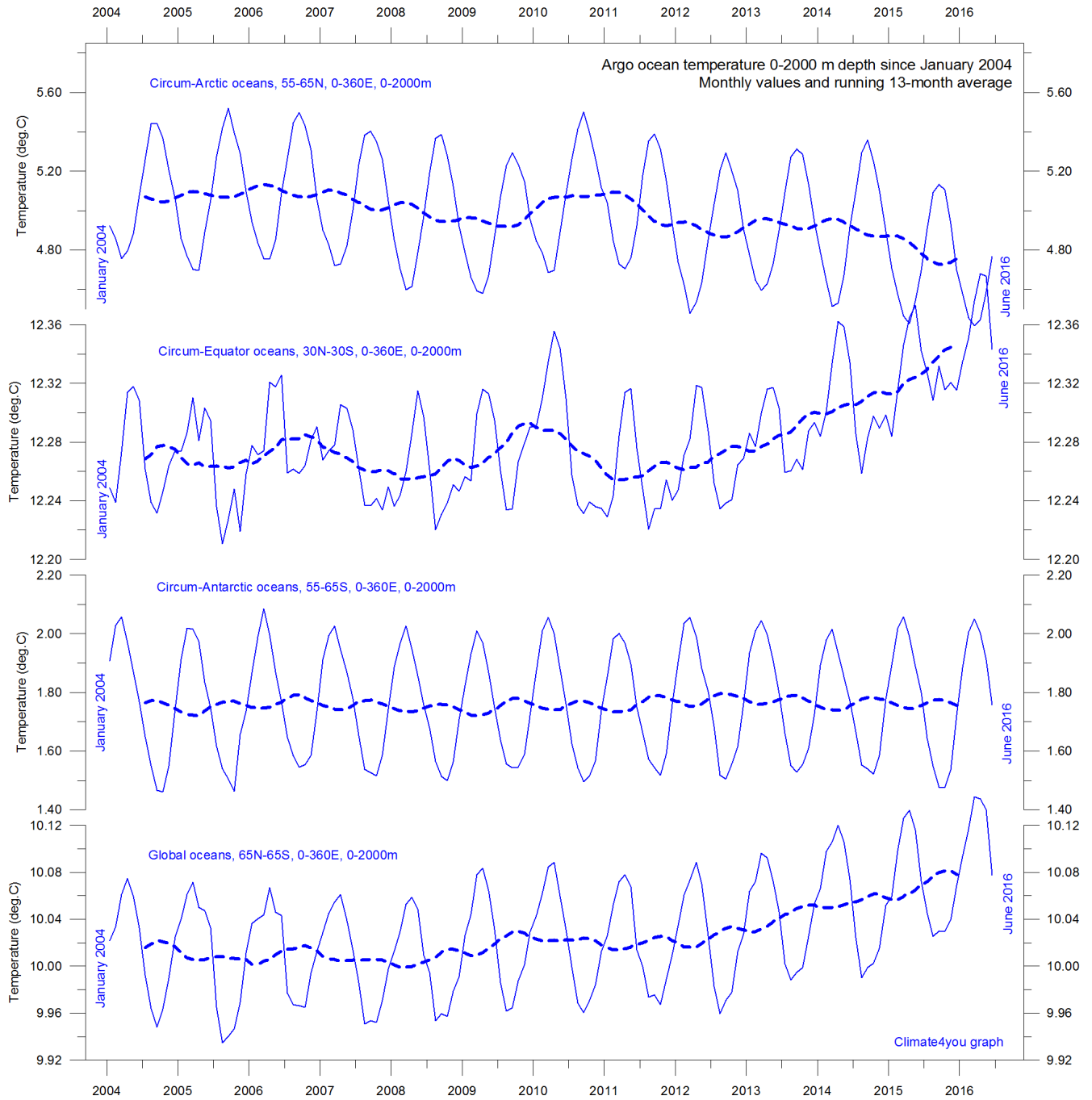
Summary of average temperature in uppermost 2000 m in different parts of the global oceans, using Argo -data. Source: Global Marine Argo Atlas . Additional information can be found in: Roemmich, D. and J. Gilson, 2009. The 2004-2008 mean and annual cycle of temperature, salinity, and steric height in the global ocean from the Argo Program. Progress in Oceanography , 82, 81-100.
