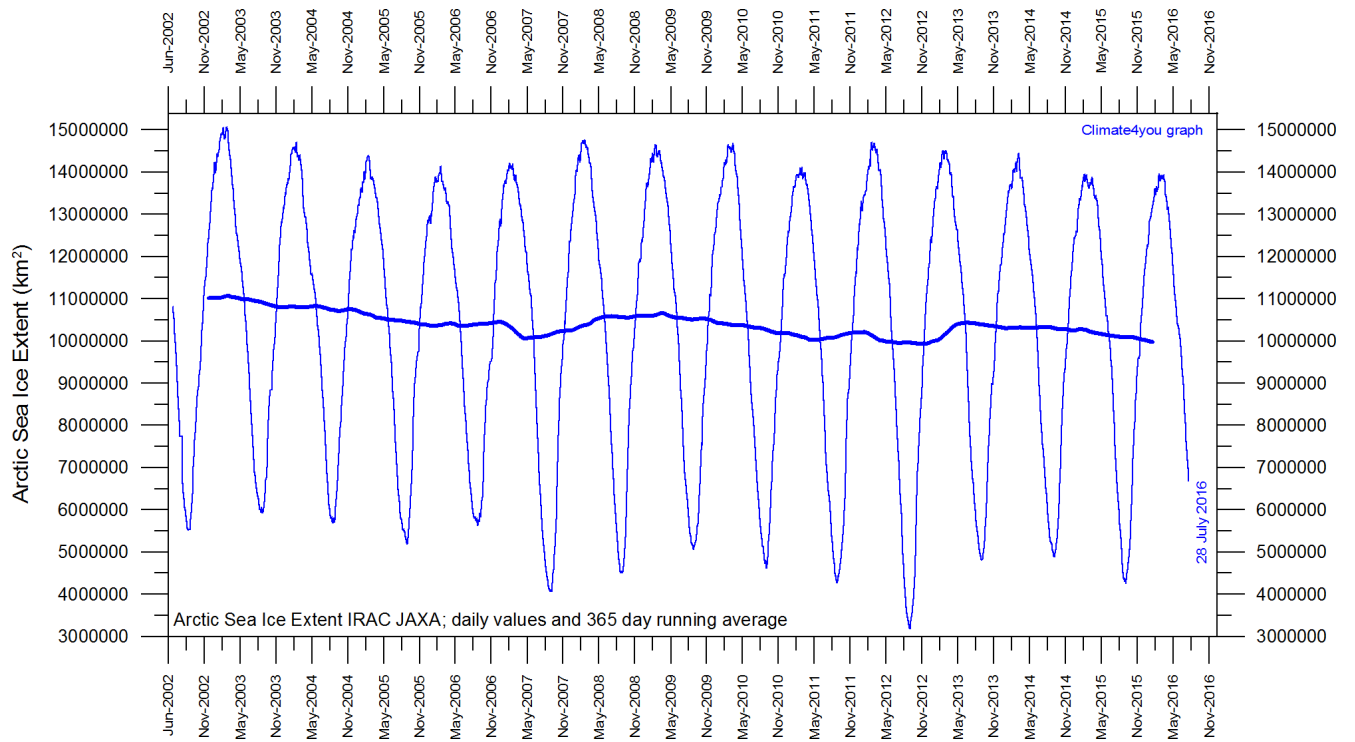
Diagram showing daily Arctic sea ice extent since June 2002, to 28 July 2016, by courtesy of Japan Aerospace Exploration Agency (JAXA) .
