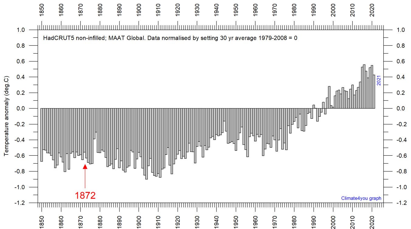
Figure 2. Anomalies of global annual surface air temperature (MAAT) since 1850 according to Hadley CRUT, a cooperative effort between the Hadley Centre for Climate Prediction and Research and the University of East Anglia's Climatic Research Unit (CRU), UK. The average for 1979-2008 (30 yrs) has been set to zero. The Baltic Sea Flood took place in a somewhat cooler global climate than now.
