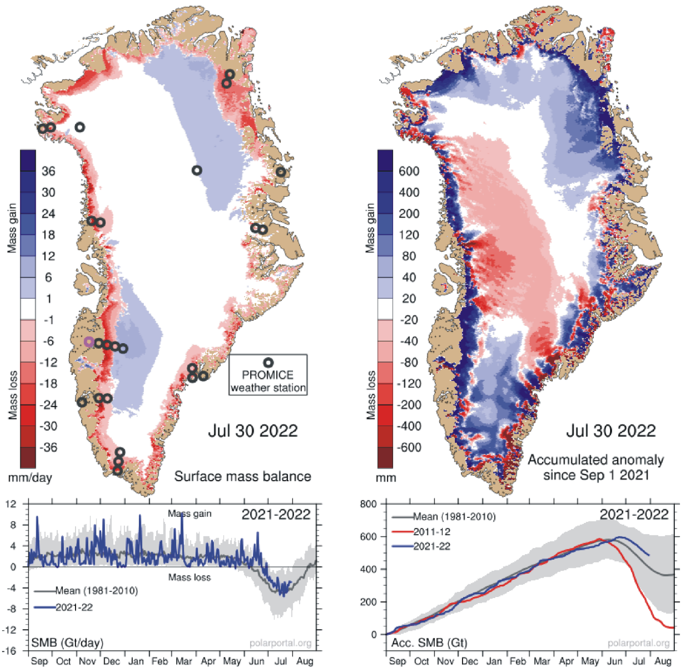
Left: Surface mass balance 30 July 2022. Right: Net surface mass balance anomaly since September 1, 2021. Courtesy of Danish Meteorological Institute (DMI).
