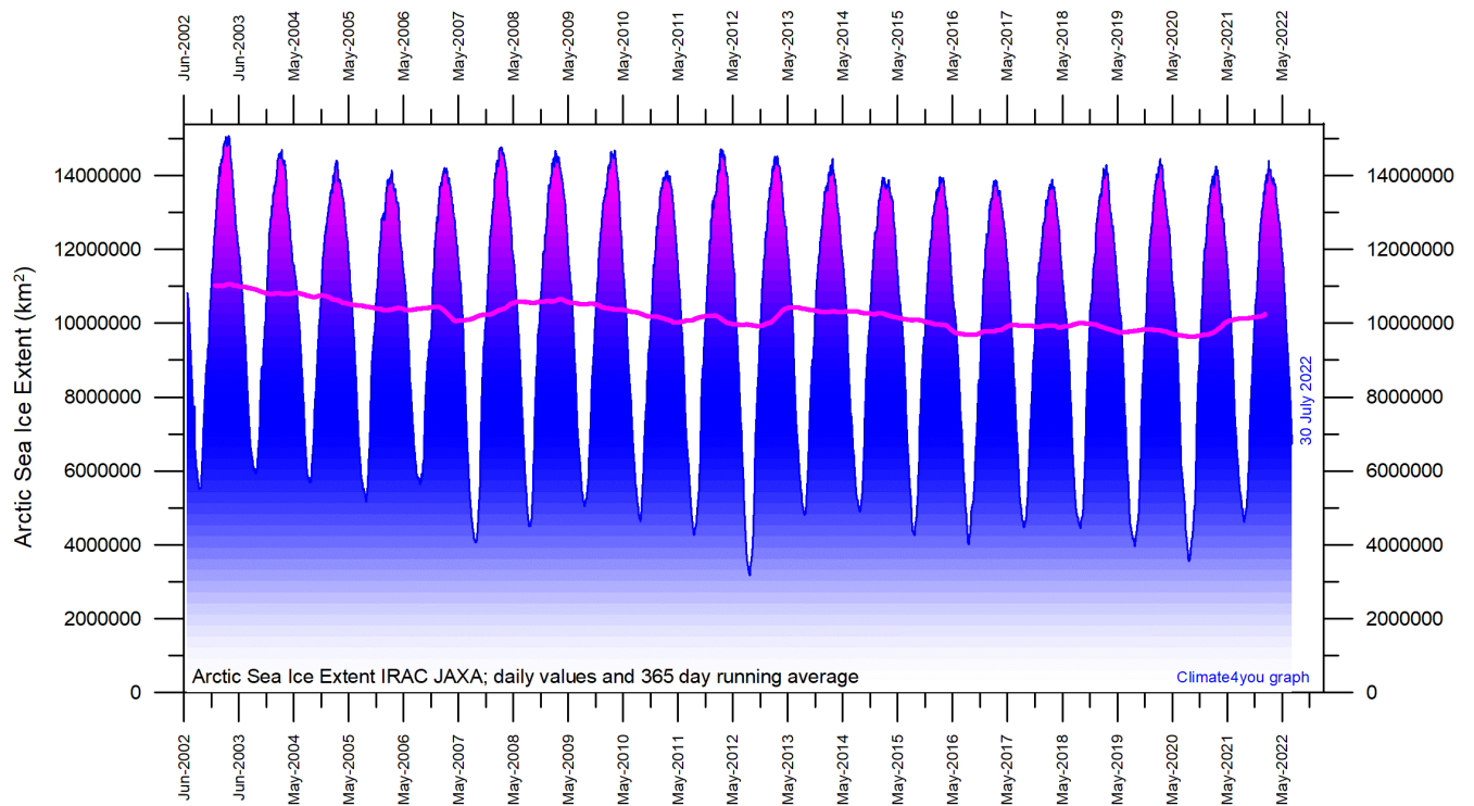
Diagram showing daily Arctic sea ice extent since June 2002, to 30 July 2022, by courtesy of Japan Aerospace Exploration Agency (JAXA).
