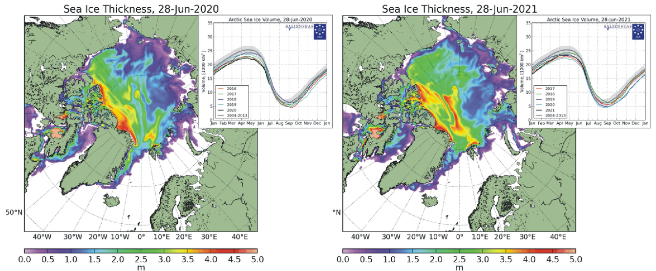
Diagrams showing Arctic sea ice extent and thickness 28 June 2020 (left) and 2021 (right and above) and the seasonal cycles of the calculated total arctic sea ice volume, according to The Danish Meteorological Institute (DMI) . The mean sea ice volume and standard deviation for the period 2004-2013 are shown by grey shading.
