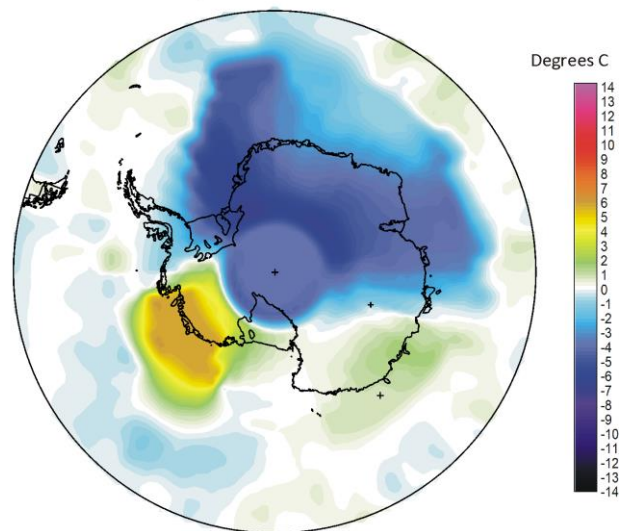
Surface air temperature June 2021 versus June 2020
