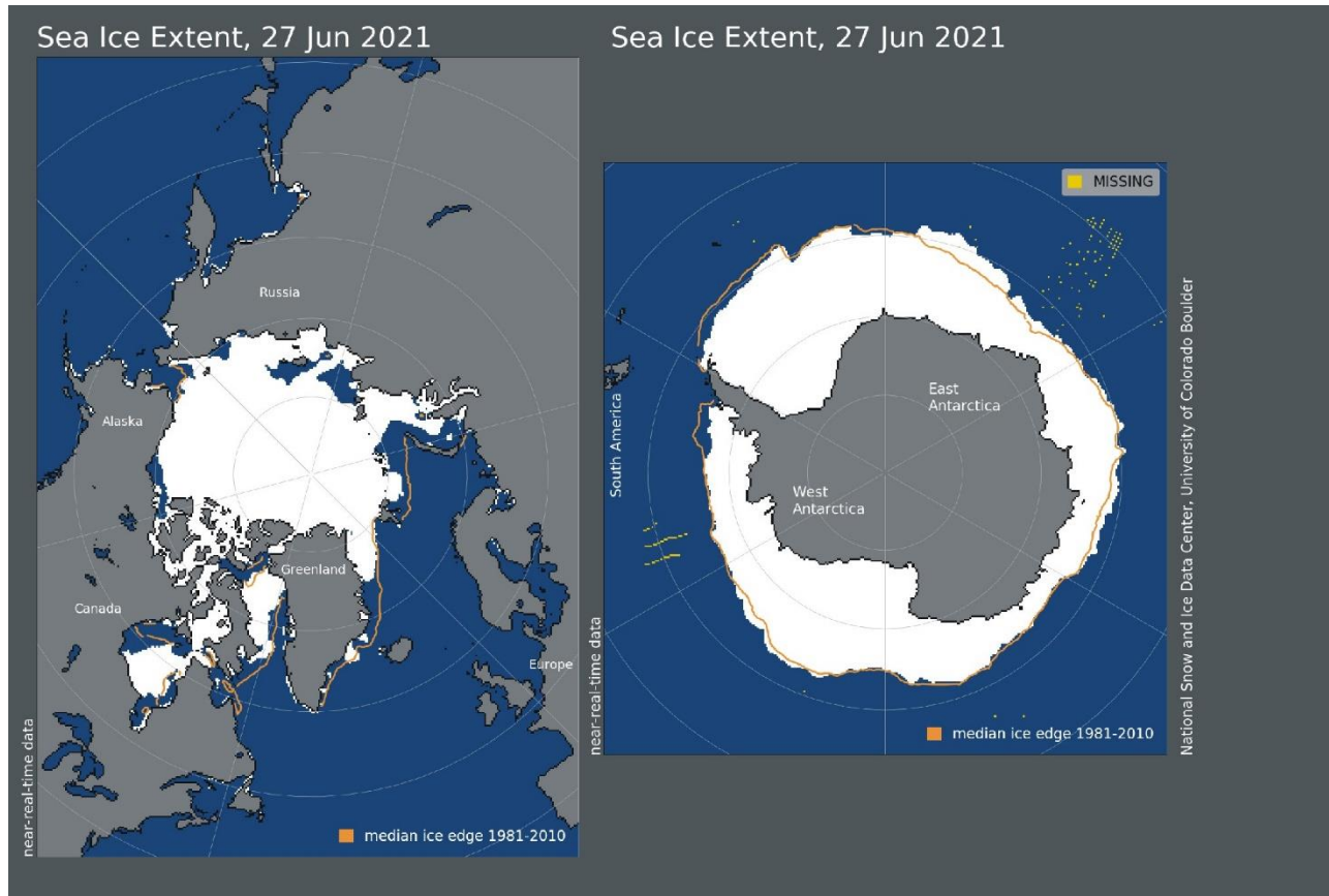
Sea ice extent 27 June 2021. The median limit of sea ice (orange line) is defined as 15% sea ice cover, according to the average of satellite observations 1981-2010 (both years included). Sea ice may therefore well be encountered outside and open water areas inside the limit shown in the diagrams above. Map source: National Snow and Ice Data Center (NSIDC).
