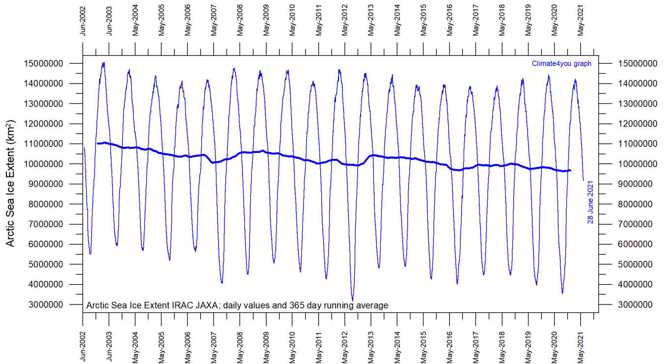
Diagram showing daily Arctic sea ice extent since June 2002, to 28 June 2021, by courtesy of Japan Aerospace Exploration Agency (JAXA) .
