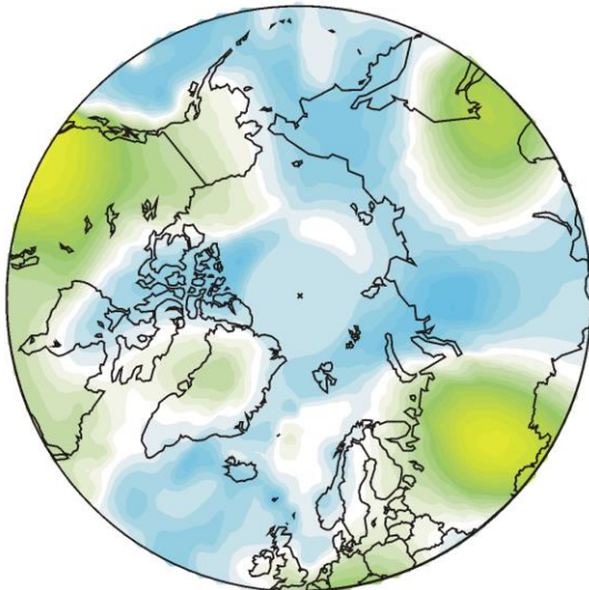
Surface air temperature June 2021 versus June 2020
