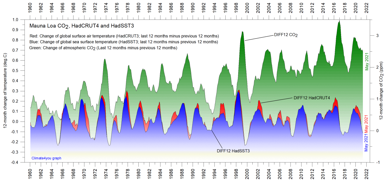
12-month change of global atmospheric CO 2 concentration ( Mauna Loa ; green), global sea surface temperature ( HadSST3 ; blue) and global surface air temperature ( HadCRUT4 ; red dotted). All graphs are showing monthly values of DIFF12, the difference between the average of the last 12 months and the average for the previous 12 months for each data series.
