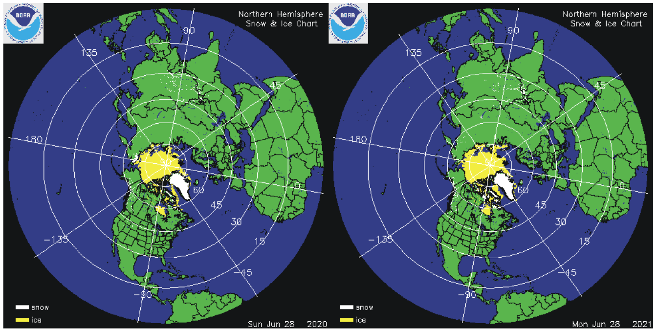
Northern hemisphere snow cover (white) and sea ice (yellow) 28 June 2020 (left) and 2021 (right). Map source: National Ice Center (NIC) .
