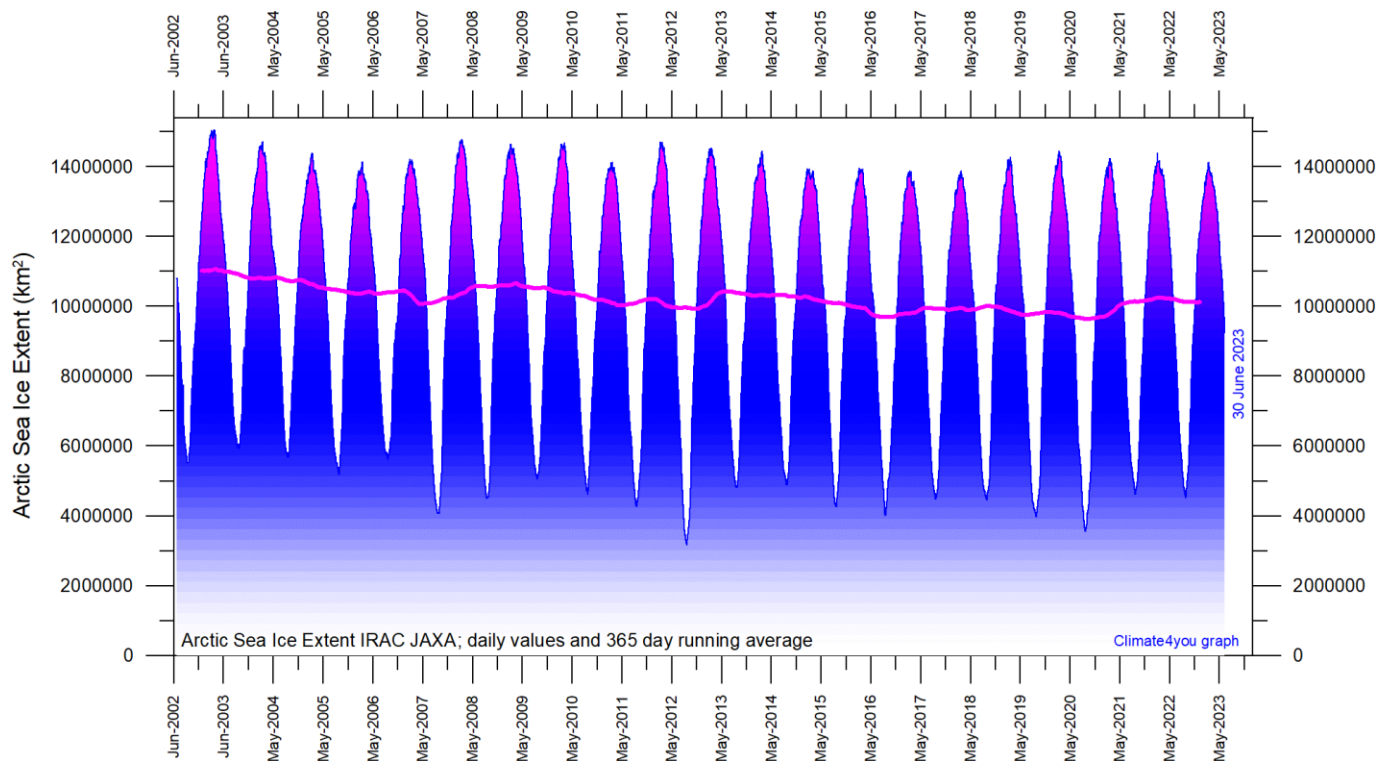
Diagram showing daily Arctic sea ice extent since June 2002, to 30 June 2023, data courtesy of Japan Aerospace Exploration Agency (JAXA) .
