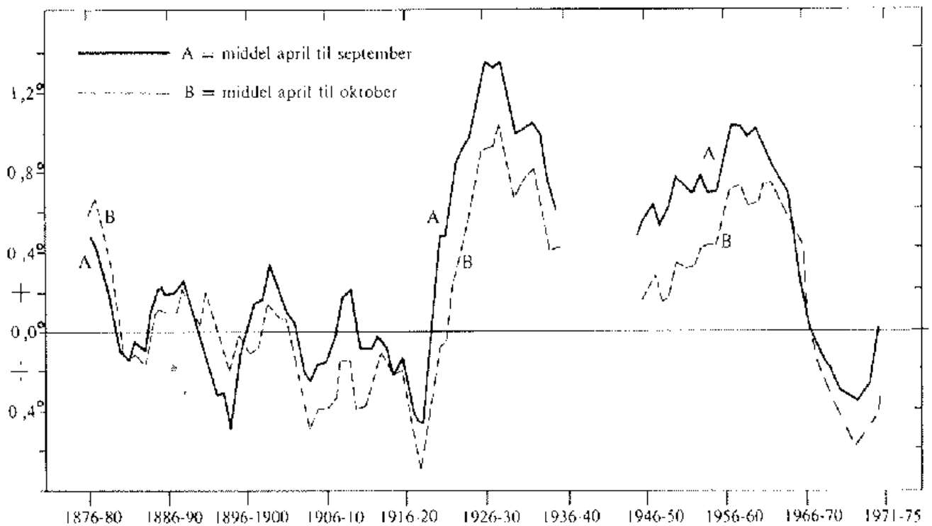
Diagram showing sea surface temperatures (degrees Centigrade, 5-yr average) along the west coast of southern Greenland (Figure 6 A in Balslev Smidt, 1989). The solid line shows the average temperature April – September, while the dotted line shows the average temperature April – October. Temperatures are shown as deviations (anomalies) from the average temperature during the relatively cold reference period 1876-1915.
