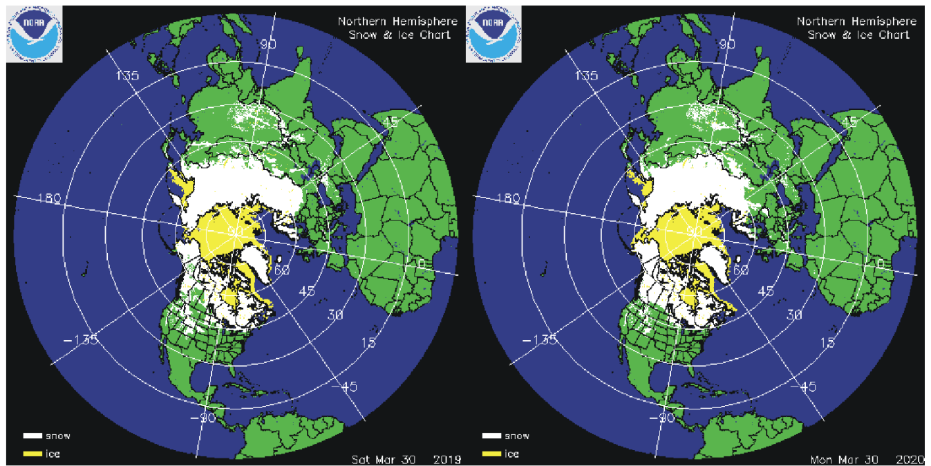
Northern hemisphere snow cover (white) and sea ice (yellow) 30 March 2019 (left) and 2020 (right). Map source: National Ice Center (NIC) .
