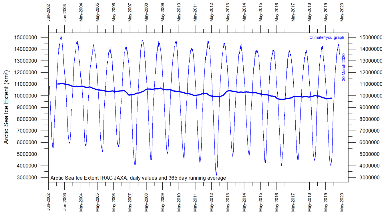
Diagram showing daily Arctic sea ice extent since June 2002, to 30 March 2020, by courtesy of Japan Aerospace Exploration Agency (JAXA).
