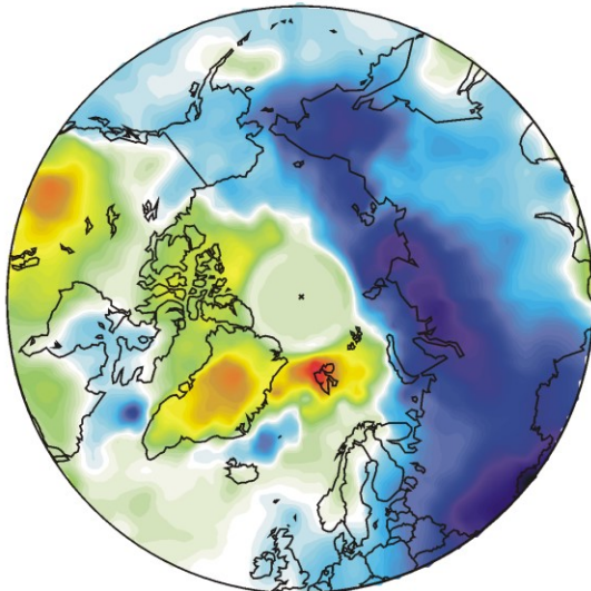
Surface air temperature March 2021 versus March 2020
