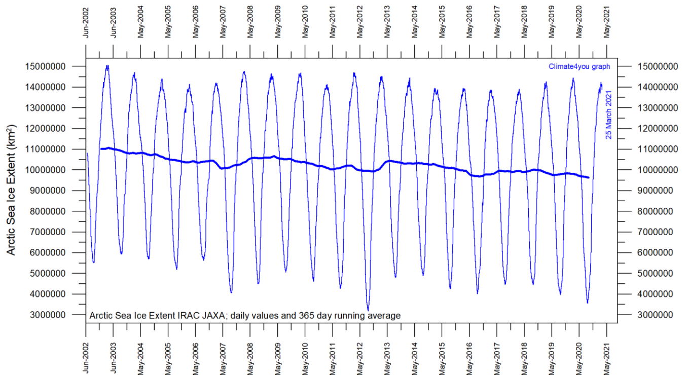
Diagram showing daily Arctic sea ice extent since June 2002, to 25 March 2021, by courtesy of Japan Aerospace Exploration Agency (JAXA).
