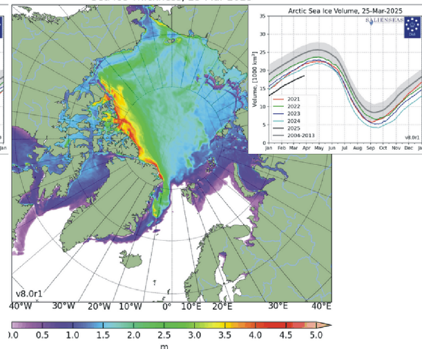
Sea Ice Thickness, 25-Mar-2025
