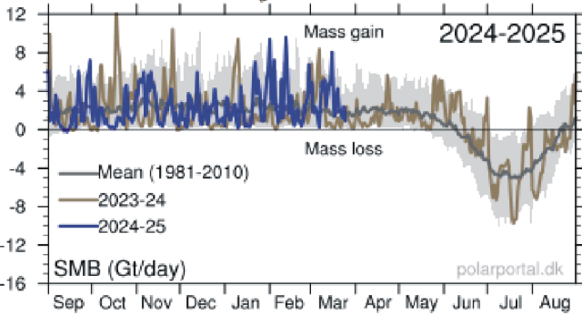
Left: Surface mass balance 25 March 2025. Right: Net surface mass balance anomaly since September 1, 2024. Courtesy of Danish Meteorological Institute (DMI).
