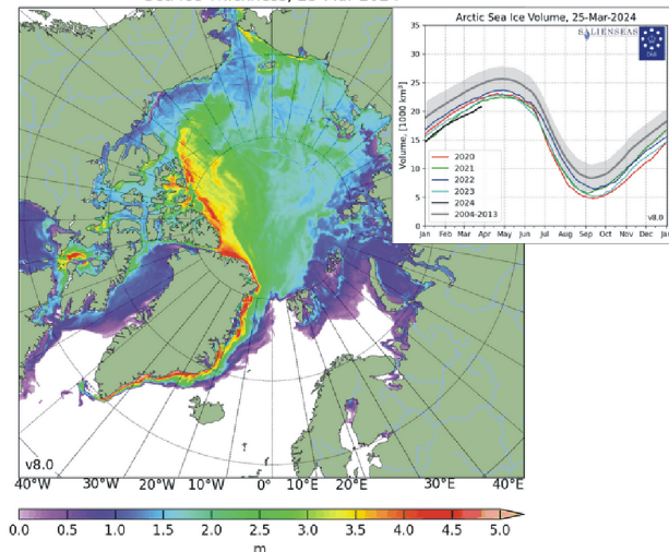
Sea Ice Thickness, 25-Mar-2024
