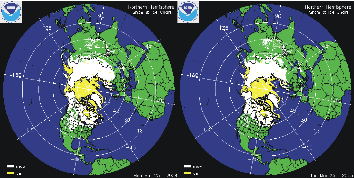
Northern hemisphere snow cover (white) and sea ice (yellow) 25 March 2024 (left) and 2025 (right). Map source: National Ice Center (NIC) .
