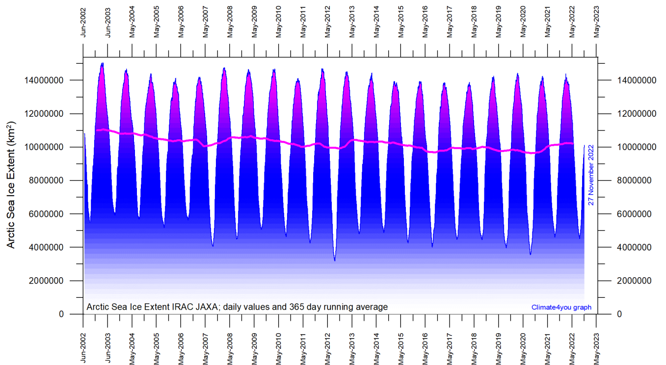
Diagram showing daily Arctic sea ice extent since June 2002, to 27 November 2022, by courtesy of Japan Aerospace Exploration Agency (JAXA).
