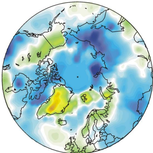
Surface air temperature November 2022 versus November last 10 yr
