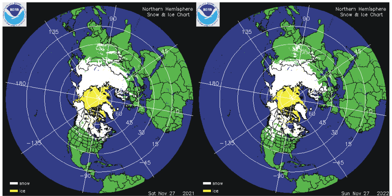
Northern hemisphere snow cover (white) and sea ice (yellow) 27 November 2021 (left) and 2022 (right). Map source: National Ice Center (NIC).
