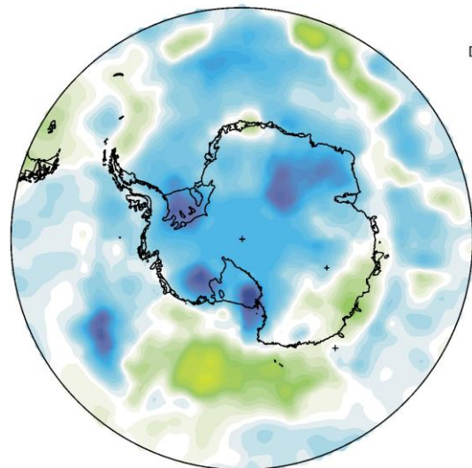
Surface air temperature November 2022 versus November 2021
