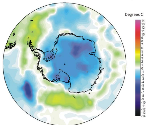
Surface air temperature November 2022 versus November last 10 yr
