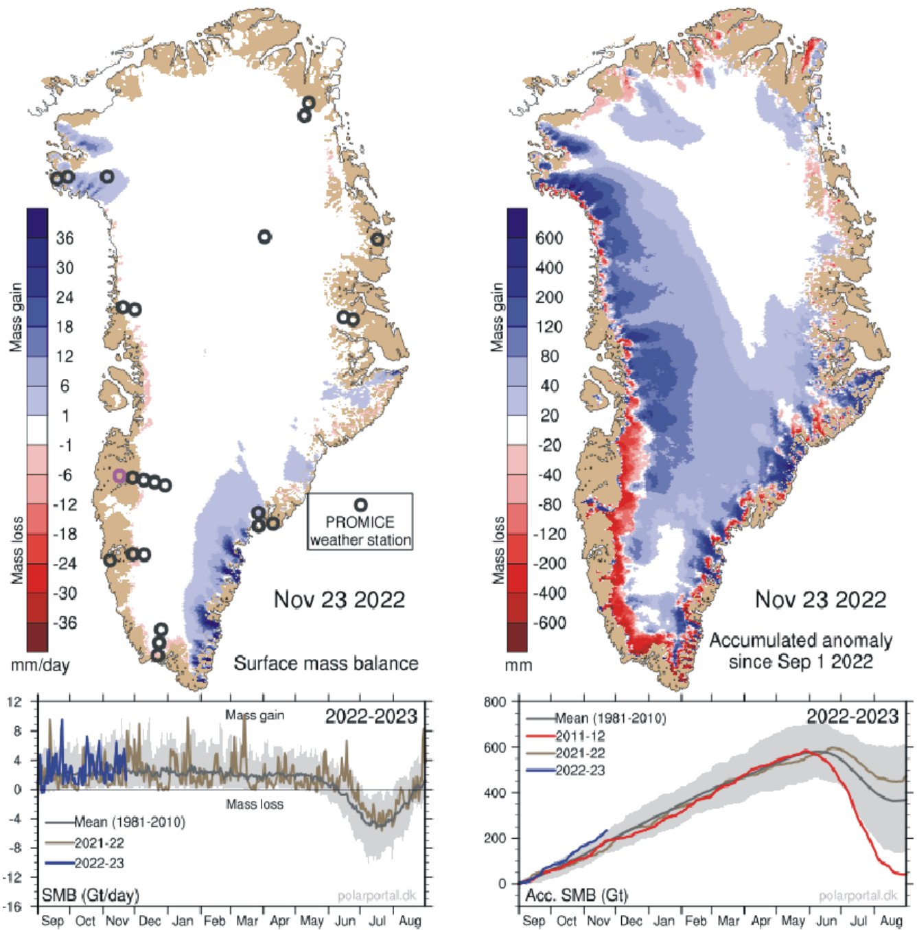
Left: Surface mass balance 23 November 2022. Right: Net surface mass balance anomaly since September 1, 2022. Courtesy of Danish Meteorological Institute (DMI).
