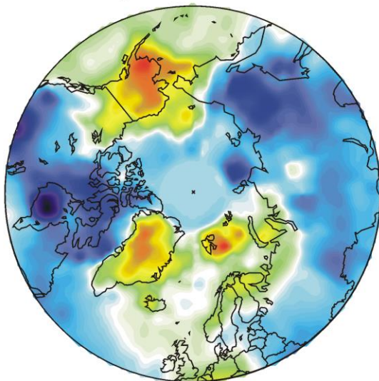
Surface air temperature November 2022 versus November 2021
