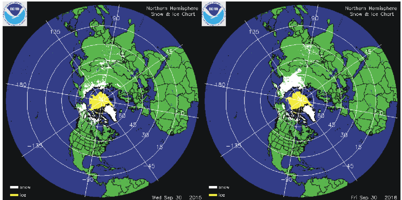
Northern hemisphere snow cover (white) and sea ice (yellow) 30 September 2015 (left) and 2016 (right). Map source: National Ice Center (NIC).
