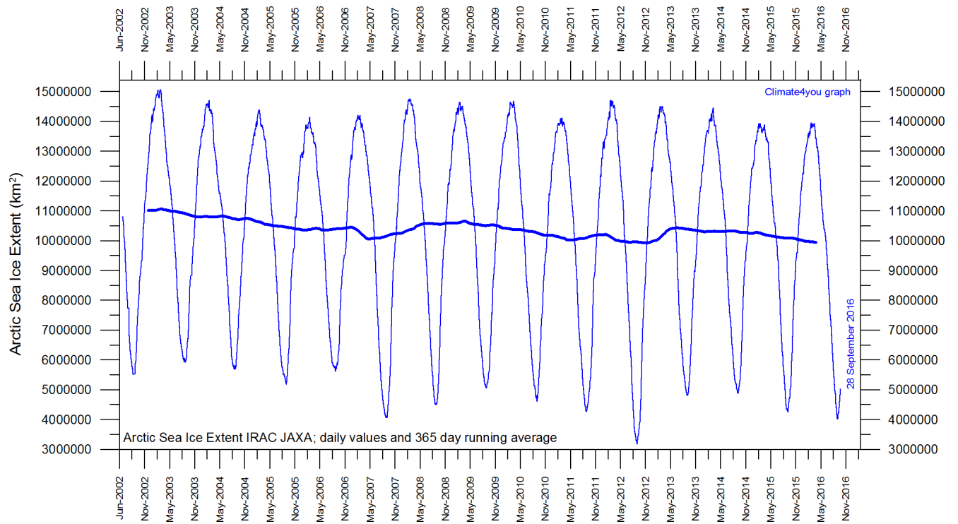
Diagram showing daily Arctic sea ice extent since June 2002, to 28 September 2016, by courtesy of Japan Aerospace Exploration Agency (JAXA) .
