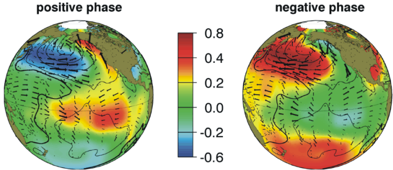
Typical wintertime Sea Surface Temperature (colors), Sea Level Pressure (black lines) and surface wind stress (arrows) anomaly patterns during warm and cool phases of PDO.
