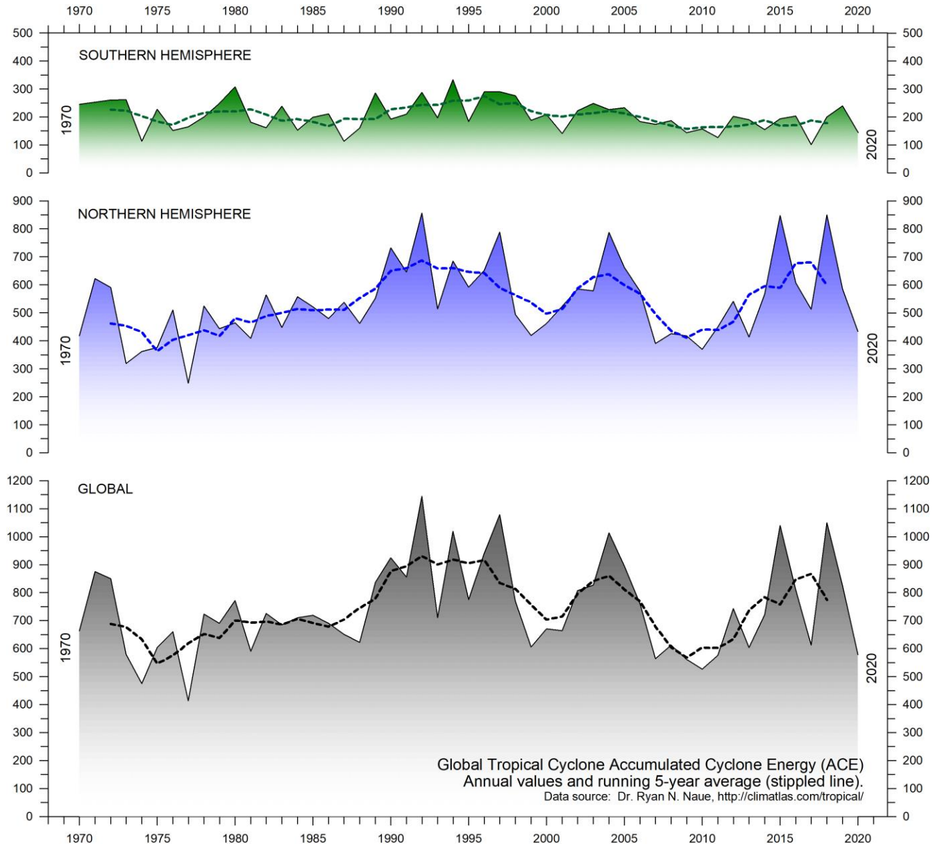
FIGURE 17: The diagram above shows the annual global tropical storm and hurricane accumulated cyclone energy (ACE) 10^4 knots 2 , since 1970. Data source: Maue ACE data.
