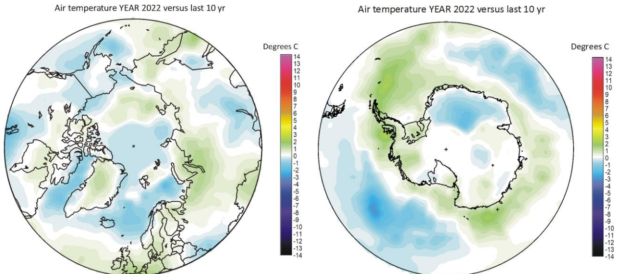
FIGURE 1. Annual 2022 average surface air temperature compared to the annual average of the last 10 years. Green-yellow-red colours indicate areas with higher temperature than the 10-year average, while blue colours indicate lower than average temperatures. Data source: Remote Sensed Surface Temperature Anomaly, AIRS/Aqua L3 Monthly Standard Physical Retrieval 1-degree x 1-degree V007 ( https://airs.jpl.nasa.gov/ ), obtained from the GISS data portal ( https://data.giss.nasa.gov/gistemp/maps/index_v4.html ).
