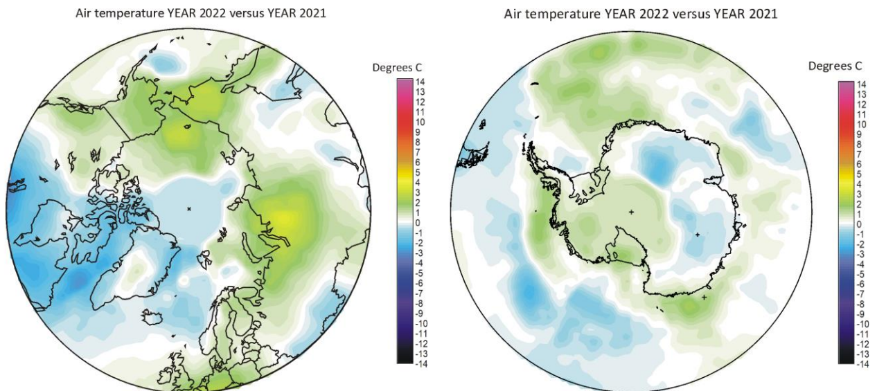
FIGURE 2. 2022 annual surface air temperature compared to year 2021. Green-yellow-red colours indicate regions where the present month was warmer than last year, while blue colours indicate regions where the present month was cooler than last year. Variations in monthly temperature from one year to the next has no tangible climatic importance but may nevertheless be interesting to study. Data source: Remote Sensed Surface Temperature Anomaly, AIRS/Aqua L3 Monthly Standard Physical Retrieval 1-degree x 1-degree V007 ( https://airs.jpl.nasa.gov/ ), obtained from the GISS data portal ( https://data.giss.nasa.gov/gistemp/maps/index_v4.html ).
