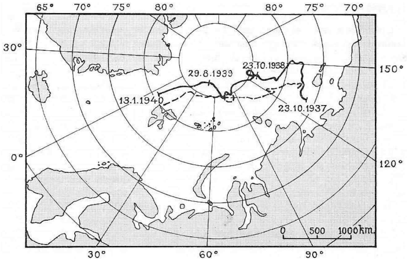
Fig. 1. Map showing the drift of the Russian icebreaker Georgi Sedow 1937-1940 (solid line) and that of the Norwegian research vessel Fram 1893-1896 (stippled line). Map source: Ahlmann 1941.
