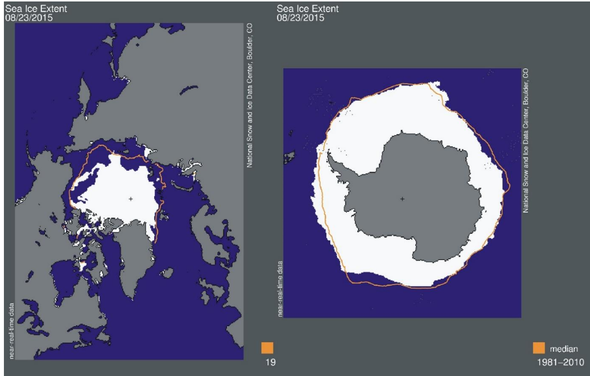
Sea ice extent 23 August 2015. The 'normal' or average limit of sea ice (orange line) is defined as 15% sea ice cover, according to the average of satellite observations 1981-2010 (both years inclusive). Sea ice may therefore well be encountered outside and open water areas inside the limit shown in the diagrams above. Map source: National Snow and Ice Data Center (NSIDC).
