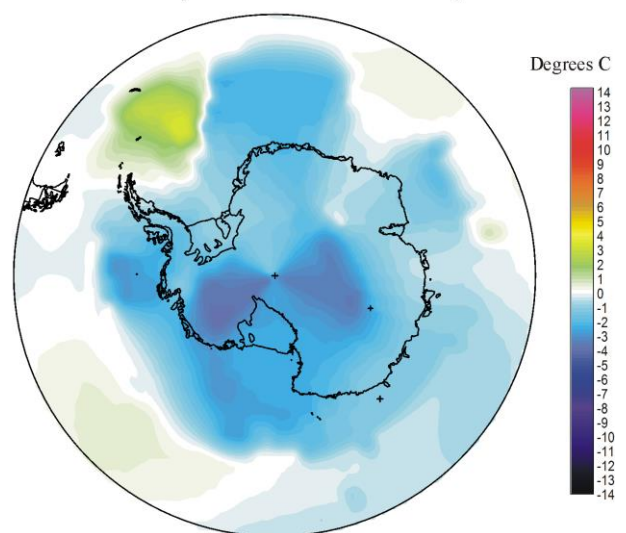
Air temperature 2015 08 versus last 10 yr
