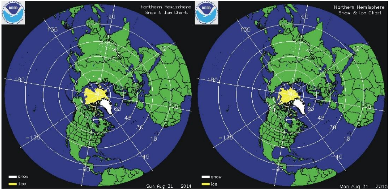
Northern hemisphere snow cover (white) and sea ice (yellow) 31 August 2014 (left) and 2015 (right). Map source: National Ice Center (NIC) .
