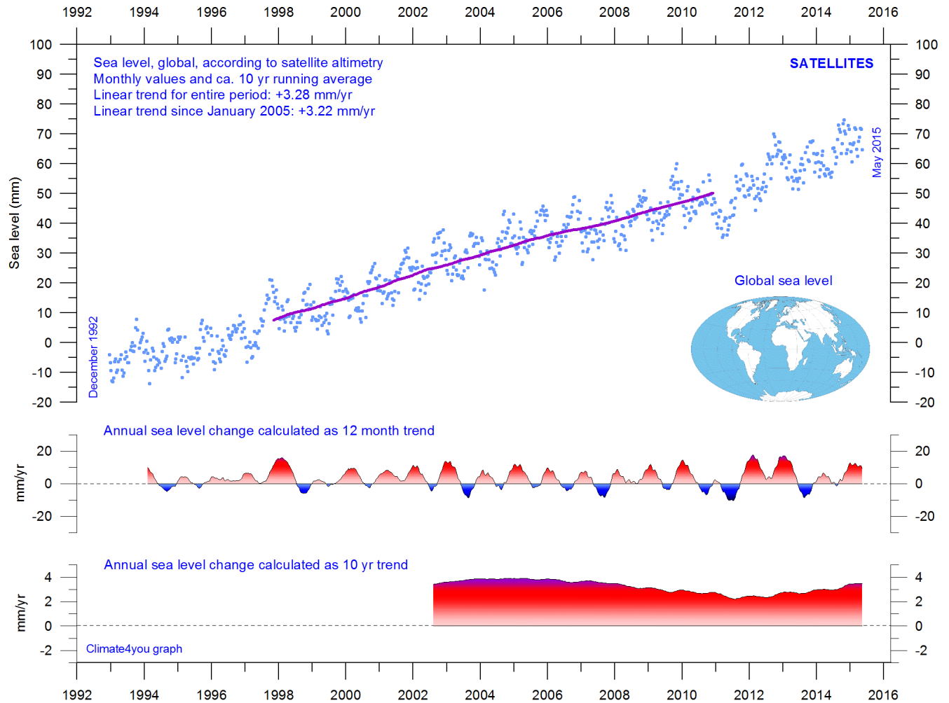
Global sea level since December 1992 according to the Colorado Center for Astrodynamic Research at University of Colorado at Boulder. The blue dots are the individual observations, and the purple line represents the running 121-month (ca. 10 year) average. The two lower panels show the annual sea level change, calculated for 1 and 10 year time windows, respectively. These values are plotted at the end of the interval considered. Data from the TOPEX/Poseidon mission have been used before 2002, and data from the Jason-1 mission (satellite launched December 2001) after 2002.
