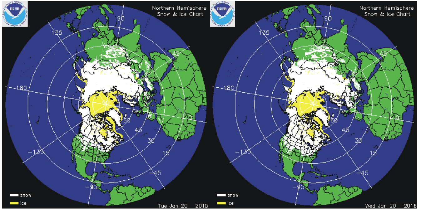
Northern hemisphere snow cover (white) and sea ice (yellow) 20 January 2015 (left) and 2016 (right). Map source: National Ice Center (NIC) .
