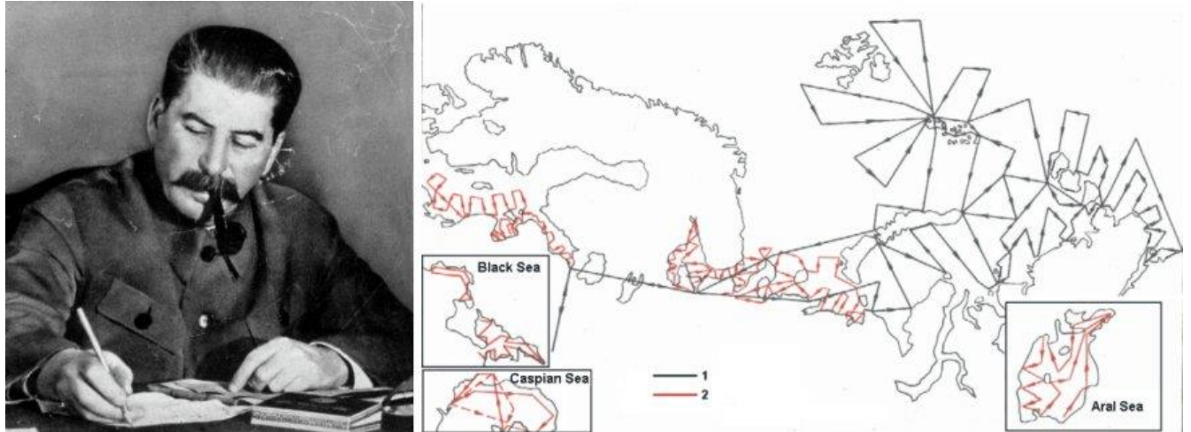
General Secretary Joseph Stalin (left). Standard airborne sea ice reconnaissance flights from 1933 (Borodachev and Shilnikov 2002). The black lines show flight paths for the air reconnaissance carried out during the season from the beginning of the programme in the last ten days of March and extending through December. The red lines show additional flight paths for the air reconnaissance carried out during the months of December, February, and March (right).
