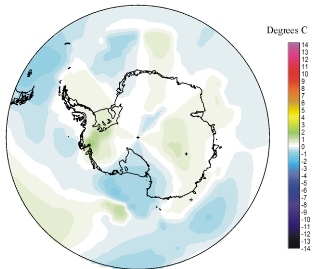
Air temperature 2015 12 versus last 10 yr
