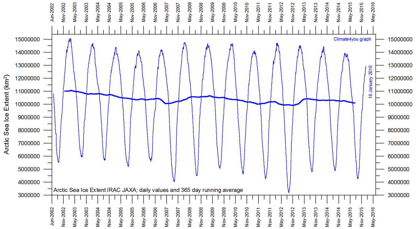
Diagram showing daily Arctic sea ice extent since June 2002, to 16 January 2016, by courtesy of Japan Aerospace Exploration Agency (JAXA) .
