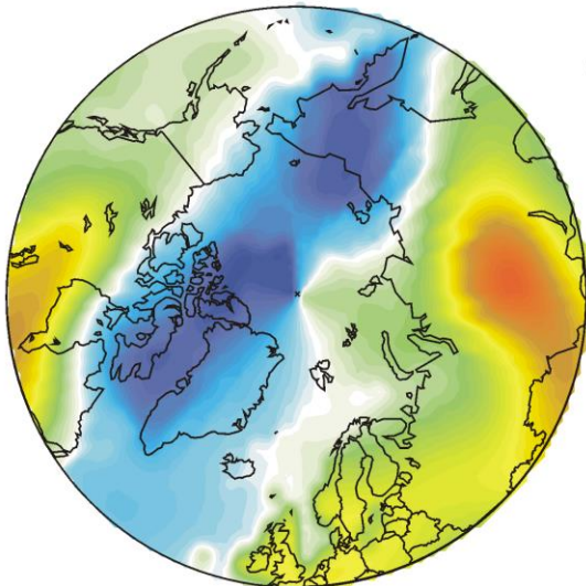
Air temperature 2015 12 versus last 10 yr
