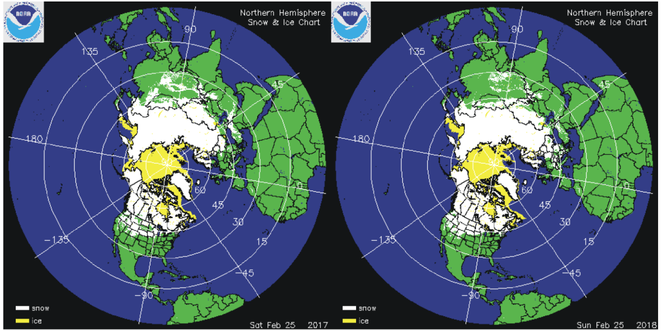
Northern hemisphere snow cover (white) and sea ice (yellow) 25 February 2017 (left) and 2018 (right). Map source: National Ice Center (NIC).
