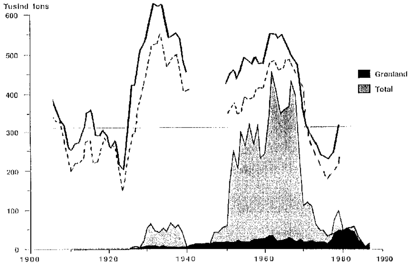
Diagram showing sea surface temperatures (degrees Centigrade) and tonnes of cod caught along the west coast of southern Greenland (Figure 6 B in Balslev Smidt, 1989). The simple 5-year average is plotted for temperatures (see diagram above). The shaded part of the diagram shows the total (grey) and the Greenlandic (black) catch, respectively. The left scale shows the catch in 1000 tonnes. During the 2nd World war no international fishing took place along West Greenland, and all cods caught was landed by Greenland vessels.
