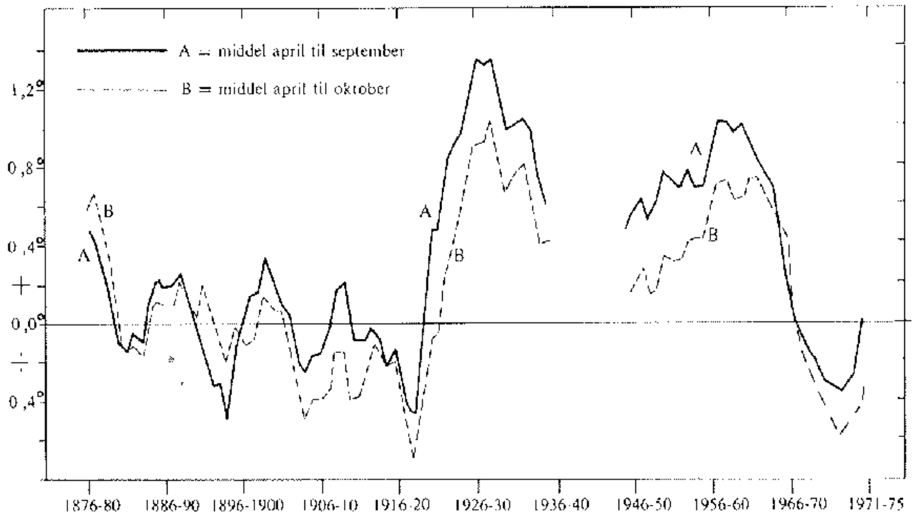
Diagram showing sea surface temperatures (degrees C) along the west coast of southern Greenland (Figure 6 A in Balslev Smidt, 1989). The simple 5-year average is plotted. The solid line shows the average temperature April – September, while the dotted line shows the average temperature April – October. Temperatures are shown as deviations (anomalies) from the average temperature during the relatively cold reference period 1876-1915.
