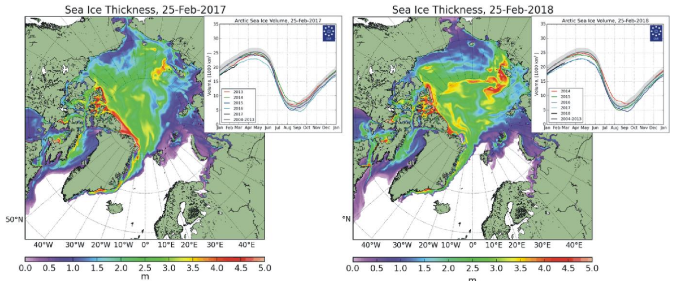
Diagrams showing Arctic sea ice extent and thickness 25 February 2017 (left) and 2018 (right and above) and the seasonal cycles of the calculated total arctic sea ice volume, according to The Danish Meteorological Institute (DMI) . The mean sea ice volume and standard deviation for the period 2004-2013 are shown by grey shading.
