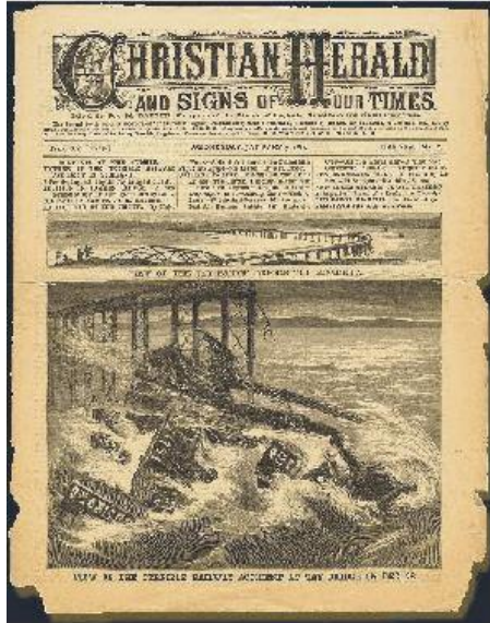
The Tay Rail Bridge disaster 28 December 1879, as documented by contemporary a contemporary newspaper (left). The old photograph to the right shows the central box-shaped section of the bridge lying on a sandbank in the river. The entire train, except for the second-class carriage and the van, was contained within this section, explaining why nobody managed to escape drowning.
