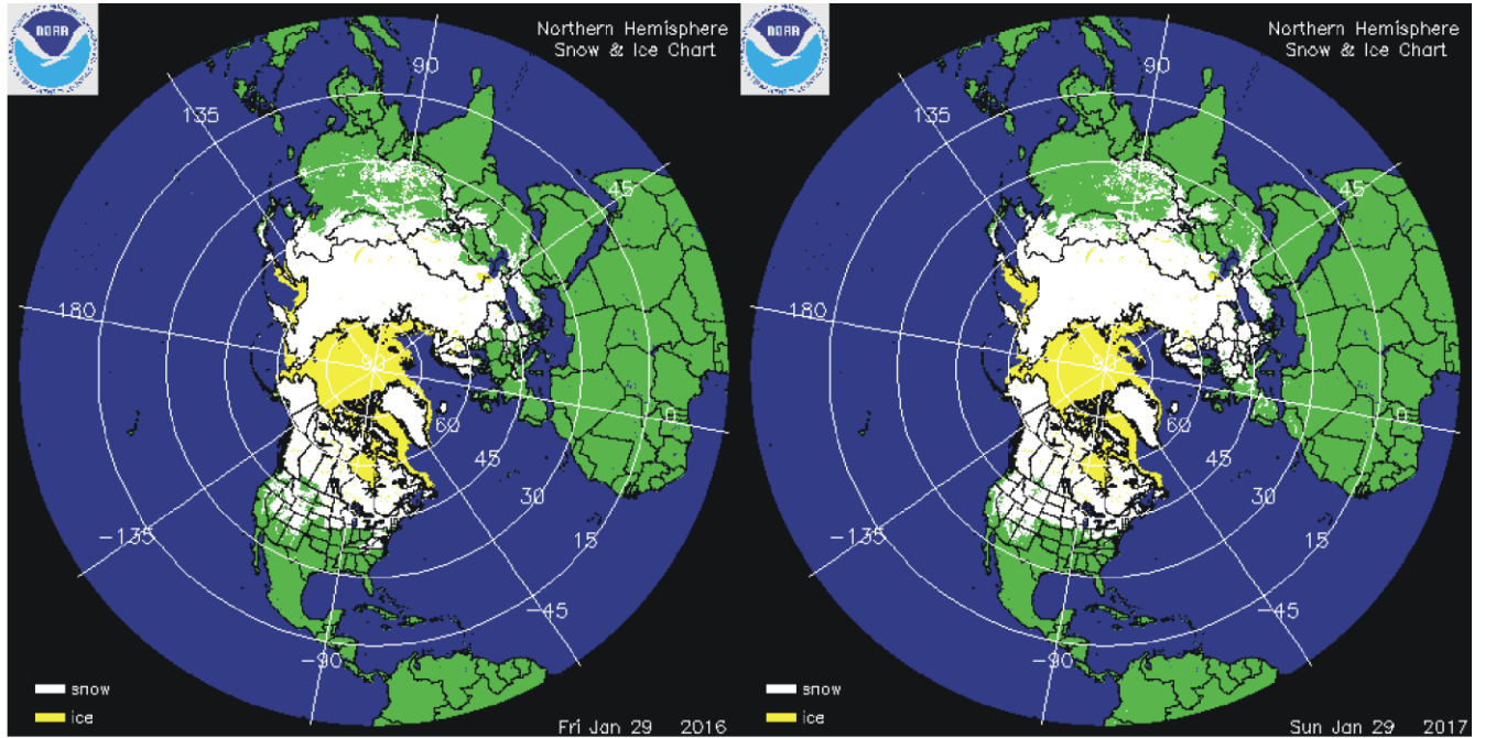
Northern hemisphere snow cover (white) and sea ice (yellow) 29 January 2016 (left) and 2017 (right). Map source: National Ice Center (NIC) .
