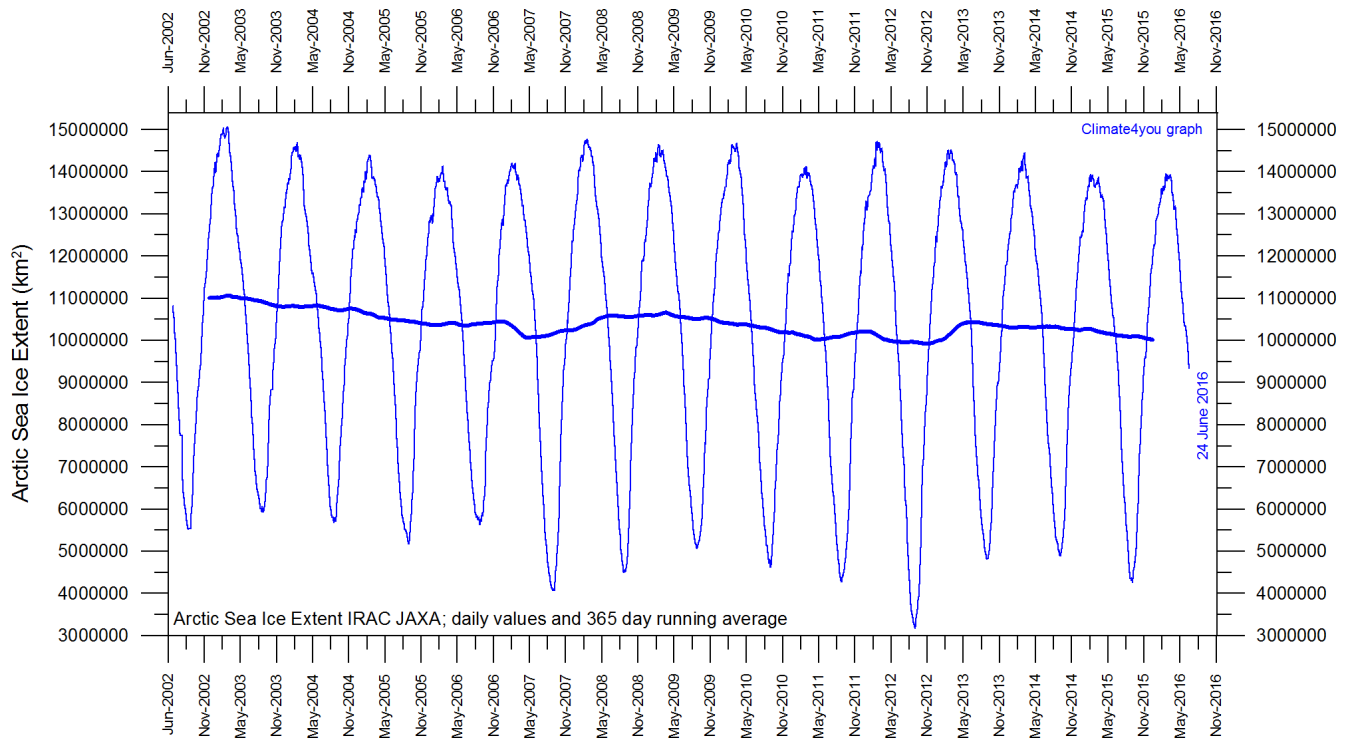
Diagram showing daily Arctic sea ice extent since June 2002, to 24 June 2016, by courtesy of Japan Aerospace Exploration Agency (JAXA) .
