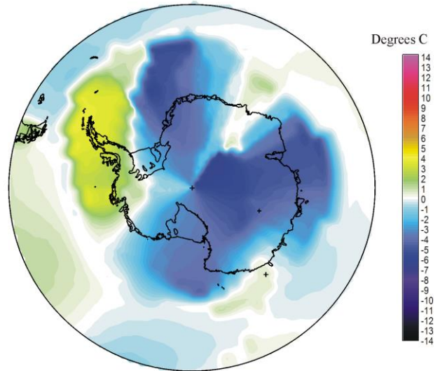
Air temperature 2016 06 versus last 10 yr
