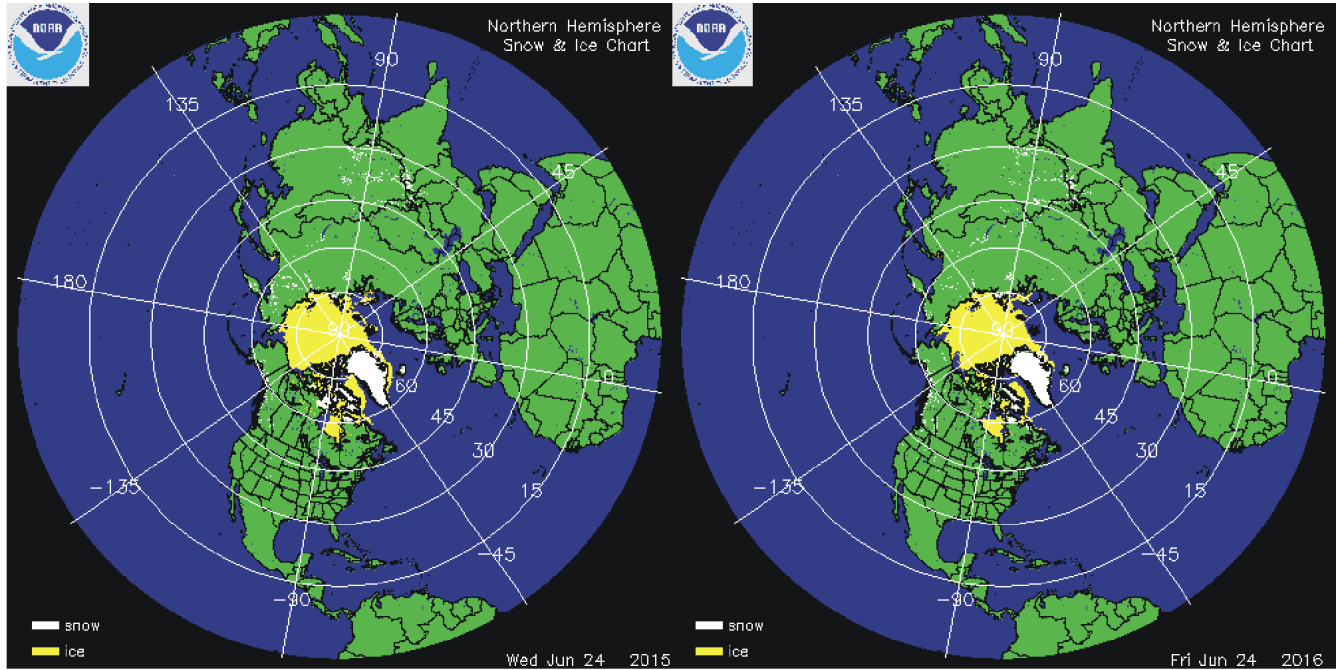
Northern hemisphere snow cover (white) and sea ice (yellow) 24 June 2015 (left) and 2016 (right). Map source: National Ice Center (NIC) .
