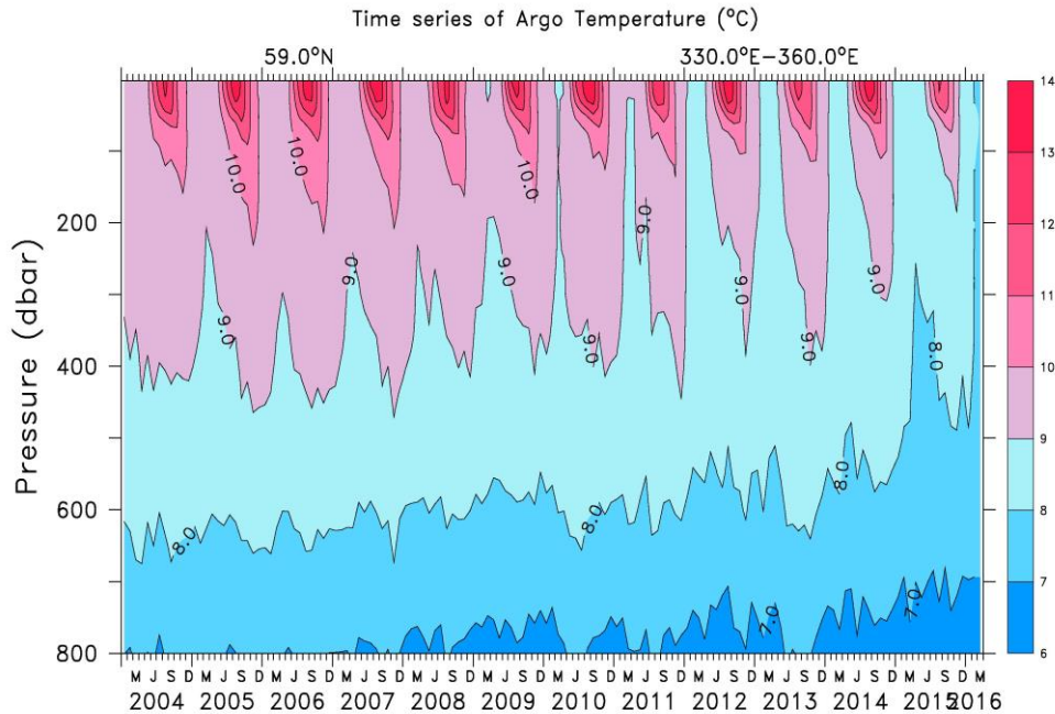
Time series depth-temperature diagram along 59 N across the North Atlantic Current from 30°W to 0°W, from surface to 800 m depth. Source: Global Marine Argo Atlas . See also the diagram below.
