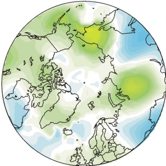
Air temperature 2016 06 versus last 10 yr
