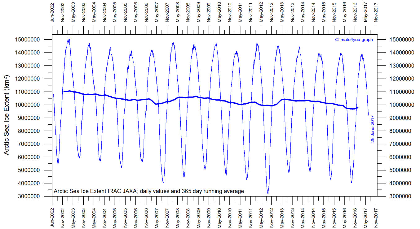
Diagram showing daily Arctic sea ice extent since June 2002, to 28 June 2017, by courtesy of Japan Aerospace Exploration Agency (JAXA) .
