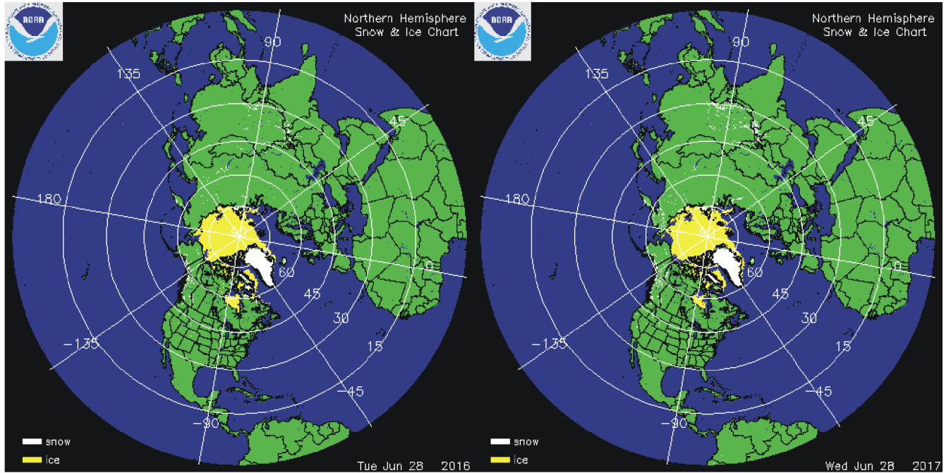
Northern hemisphere snow cover (white) and sea ice (yellow) 28 June 2016 (left) and 2017 (right). Map source: National Ice Center (NIC) .
