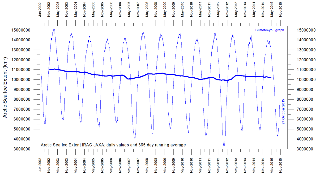
Diagram showing daily Arctic sea ice extent since June 2002, to 27 October 2015, by courtesy of Japan Aerospace Exploration Agency (JAXA) .
