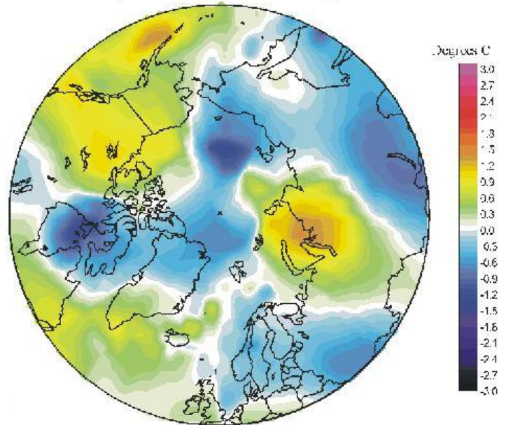
Air temperature 1942 06-08 versus average 1900-1929
