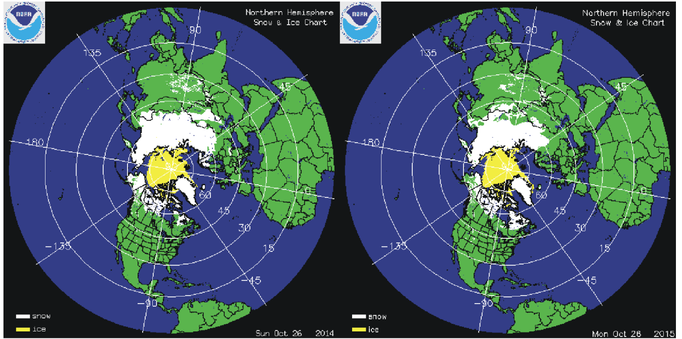
Northern hemisphere snow cover (white) and sea ice (yellow) 26 October 2014 (left) and 2015 (right). Map source: National Ice Center (NIC) .
