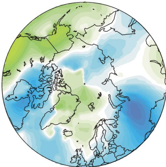
Air temperature 2015 10 versus last 10 yr
