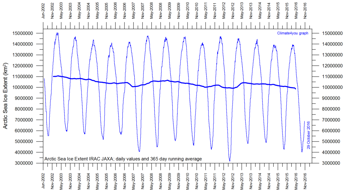
Diagram showing daily Arctic sea ice extent since June 2002, to 29 October 2016, by courtesy of Japan Aerospace Exploration Agency (JAXA) .
