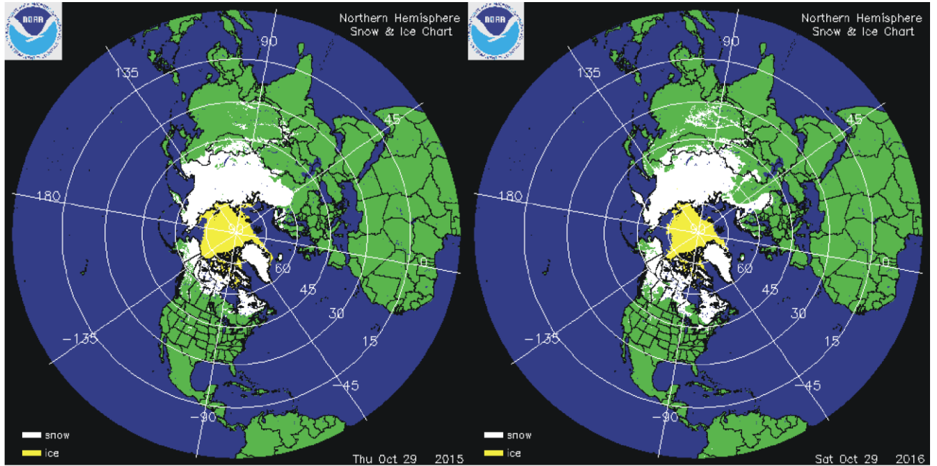
Northern hemisphere snow cover (white) and sea ice (yellow) 29 October 2015 (left) and 2016 (right). Map source: National Ice Center (NIC).
