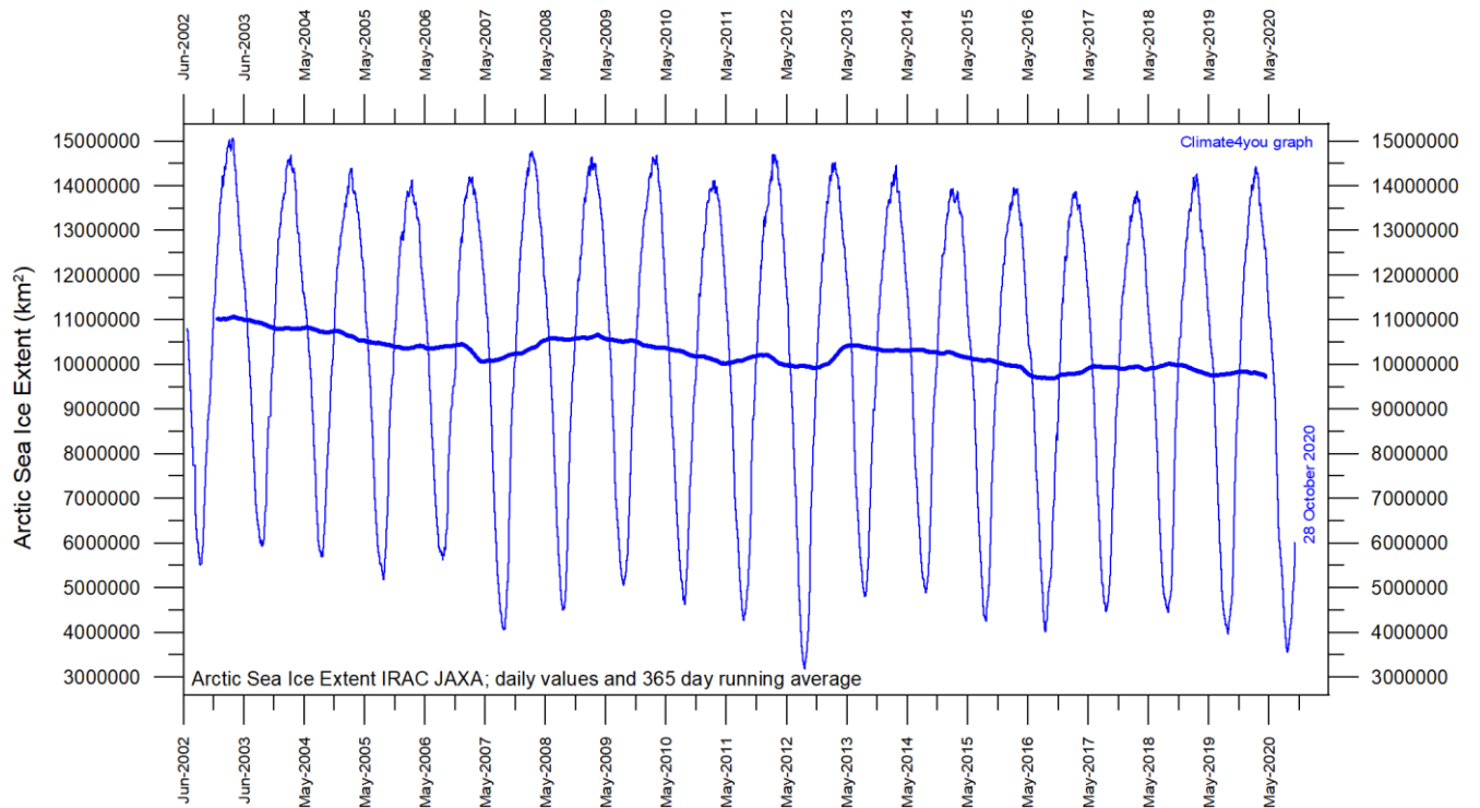
Diagram showing daily Arctic sea ice extent since June 2002, to 28 October 2020, by courtesy of Japan Aerospace Exploration Agency (JAXA) .
