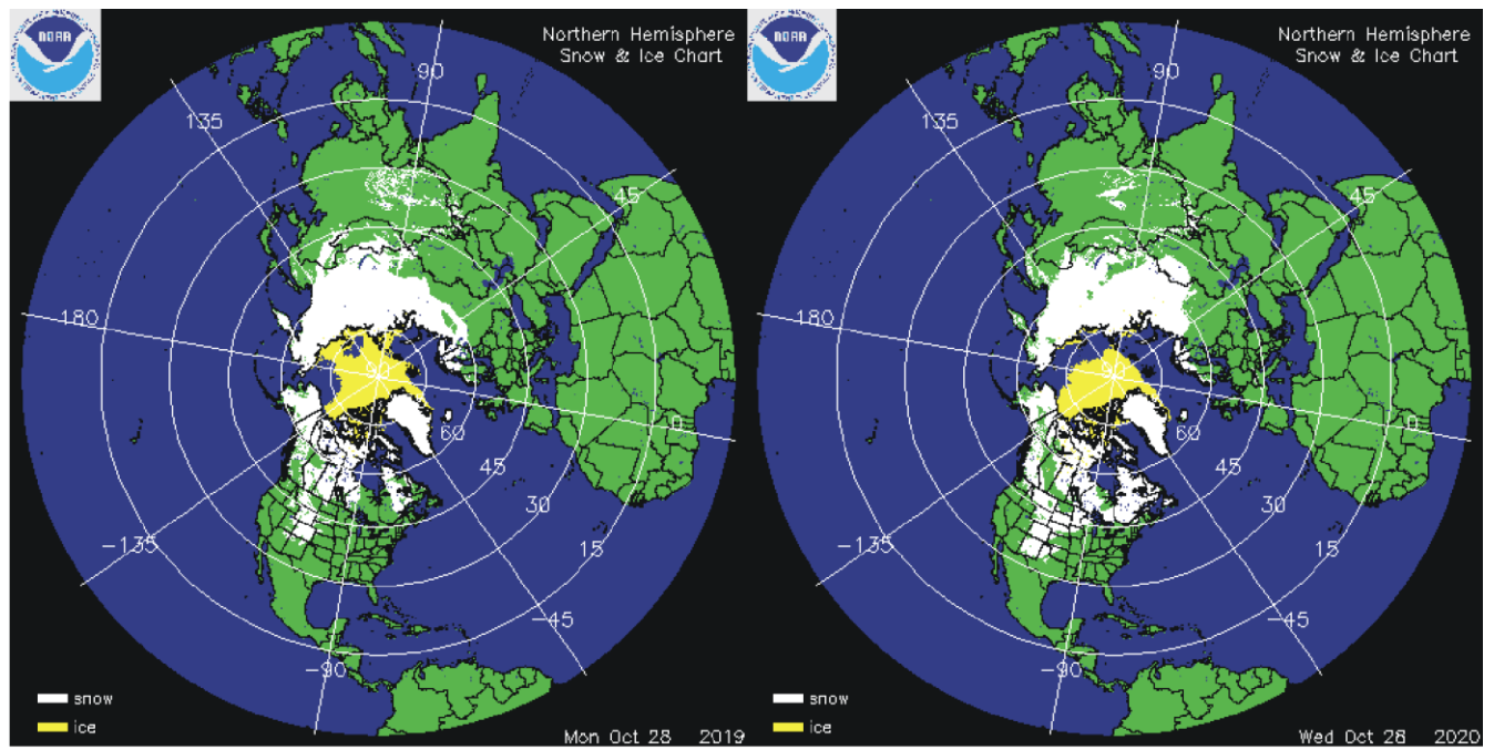
Northern hemisphere snow cover (white) and sea ice (yellow) 28 October 2019 (left) and 2020 (right). Map source: National Ice Center (NIC) .
