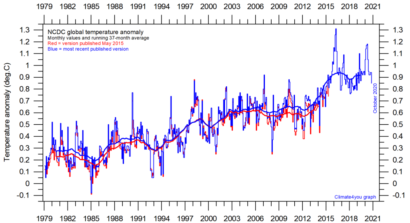
8 Global monthly average surface air temperature since 1979 according to according to the National Climatic Data Center (NCDC) , USA. The thick line is the simple running 37-month average.
