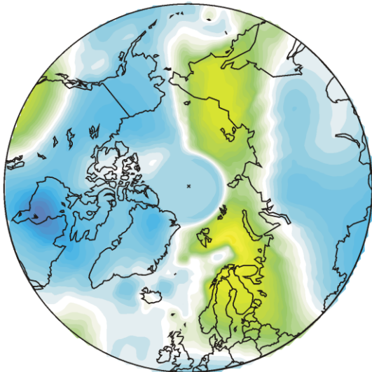
Surface air temperature October 2020 versus October 2019
