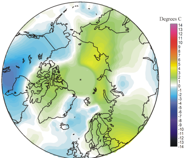
Surface air temperature October 2020 versus October last 10 yr
