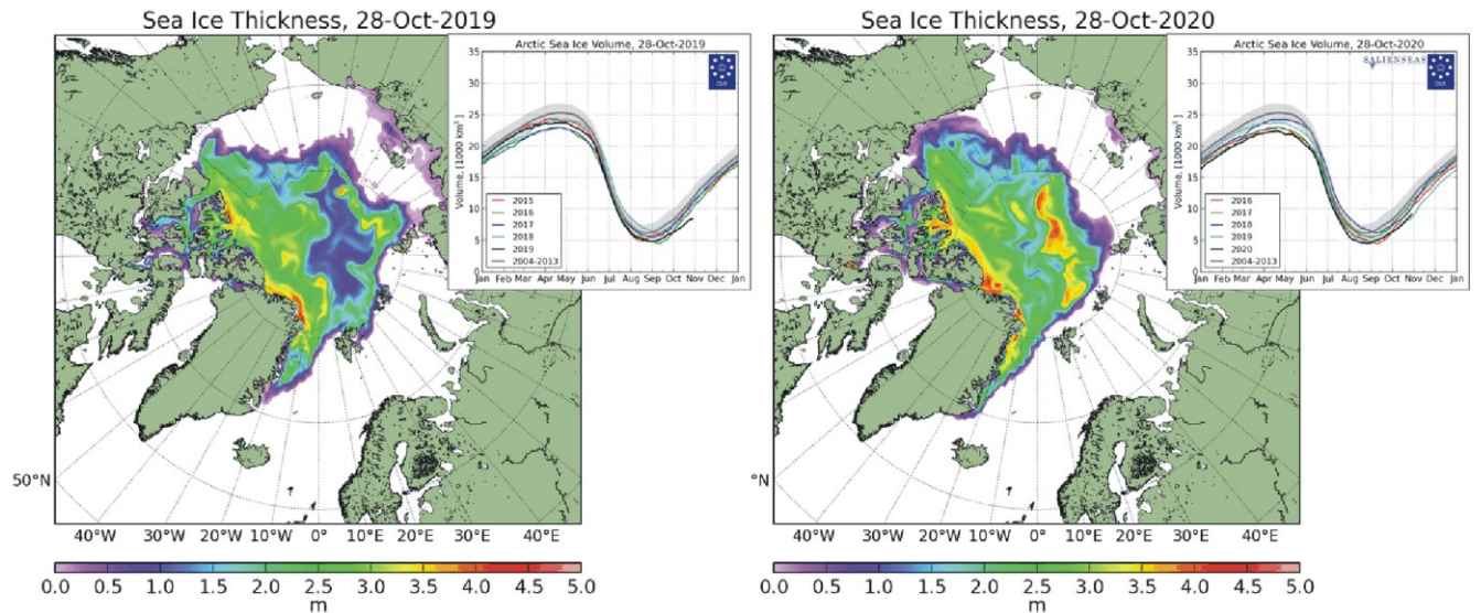
Diagrams showing Arctic sea ice extent and thickness 28 October 2019 (left) and 2020 (right and above) and the seasonal cycles of the calculated total arctic sea ice volume, according to The Danish Meteorological Institute (DMI) . The mean sea ice volume and standard deviation for the period 2004-2013 are shown by grey shading.
