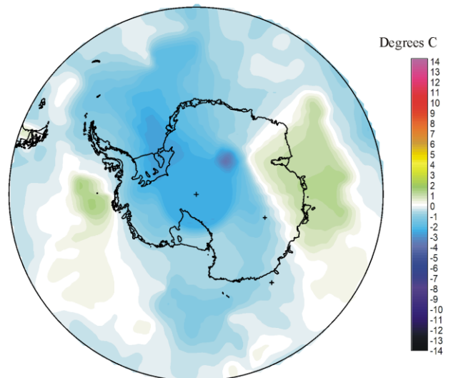
Surface air temperature October 2020 versus October last 10 yr
