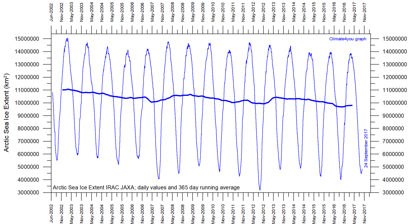
Diagram showing daily Arctic sea ice extent since June 2002, to 24 September 2017, by courtesy of Japan Aerospace Exploration Agency (JAXA) .
