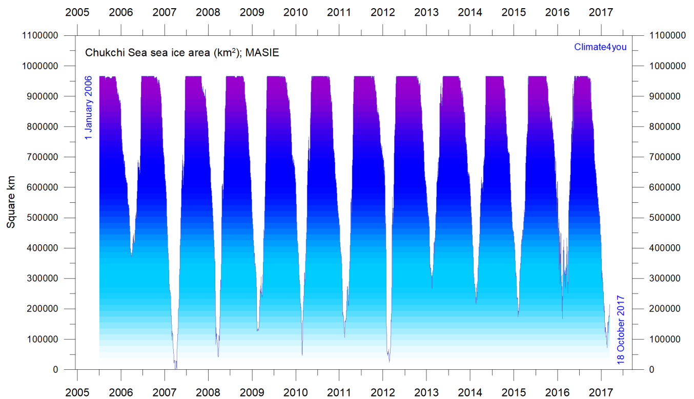
Daily sea ice extension in the Chukchi Sea according to Multisensor Analyzed Sea Ice Extent (MASIE; 2017).
